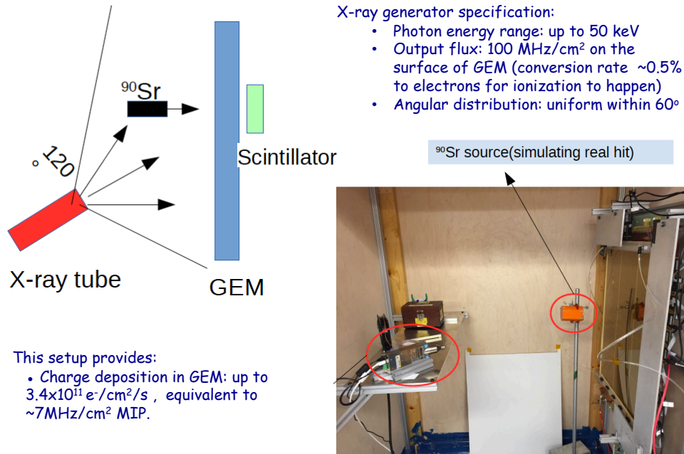
Figure 13: The UVa X-ray test setup
