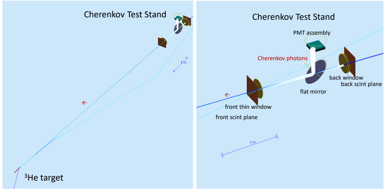
Figure 7: Simulation of the TCD in JLab Hall C. The left plot shows an electron (blue) from the polarized ^3\text{He} target entering the TCD at about 10m and 4 deg. Cherenkov lights (white) are produced by the electron, reflected on a mirror and collected by an MaPMT array. The right plot shows the same setup with zooming in on the device. The tank wall is invisible so that the internal components like the mirror and MaPMT array can be seen.
