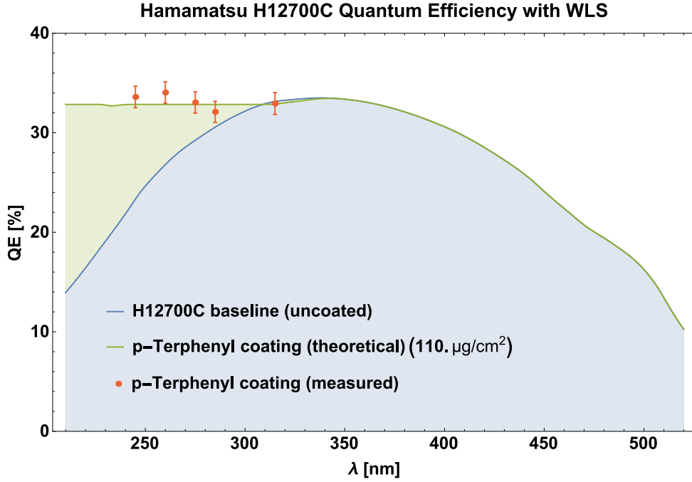
Figure 9: Nominal quantum efficiency as a function of wavelength for H12700C MaPMTs with (green) and without (blue) p-Terphenyl wavelength shifter. The red markers shows the quantum efficiency for a coated MaPMT as measured with monochromatic LEDs.
