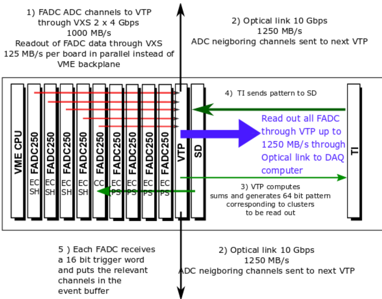
Figure 3: VXS crate module configuration for PVDIS
