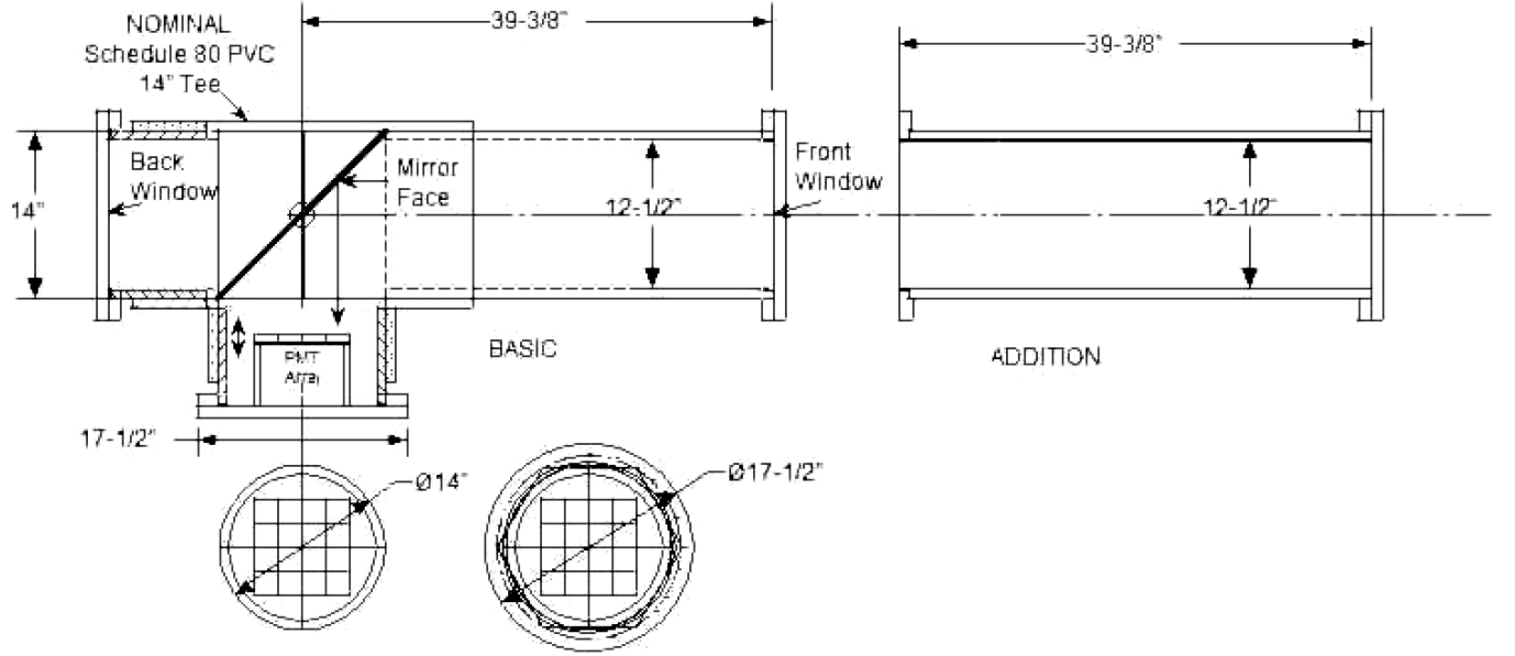
Figure 8: Tank design for the telescopic Cherenkov device.
