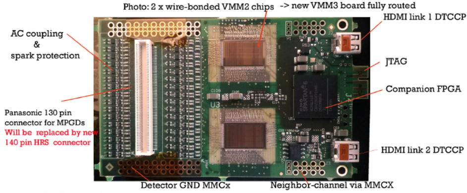
Figure 2: The VMM chip based CERN RD-51 SRS readout card. The previous generations of this readout card were based on the APV-25 chip.
