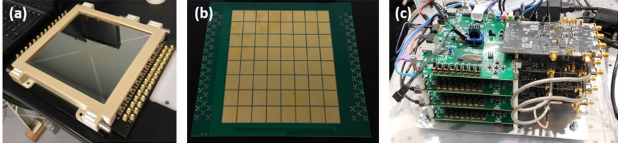
Figure 10: (a) The 20x20 cm 2 LAPPD device, and (b) 8x8 array, 25x25mm 2 , 64-pixel readout. (c) The Nalu ASoC data acquisition system, each evaluation board has 4 readout and attached to one FPGA, evaluation boards can be stack together for multi-pixel readout.
