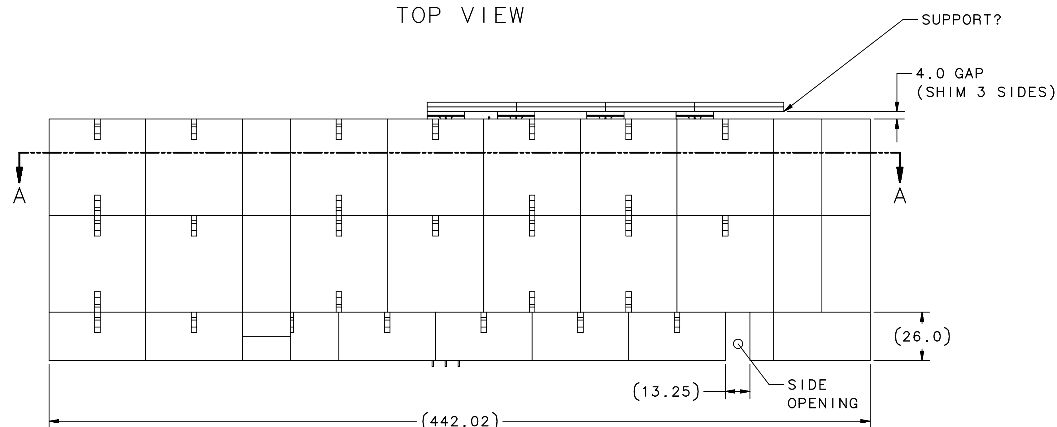
LS VIEW
