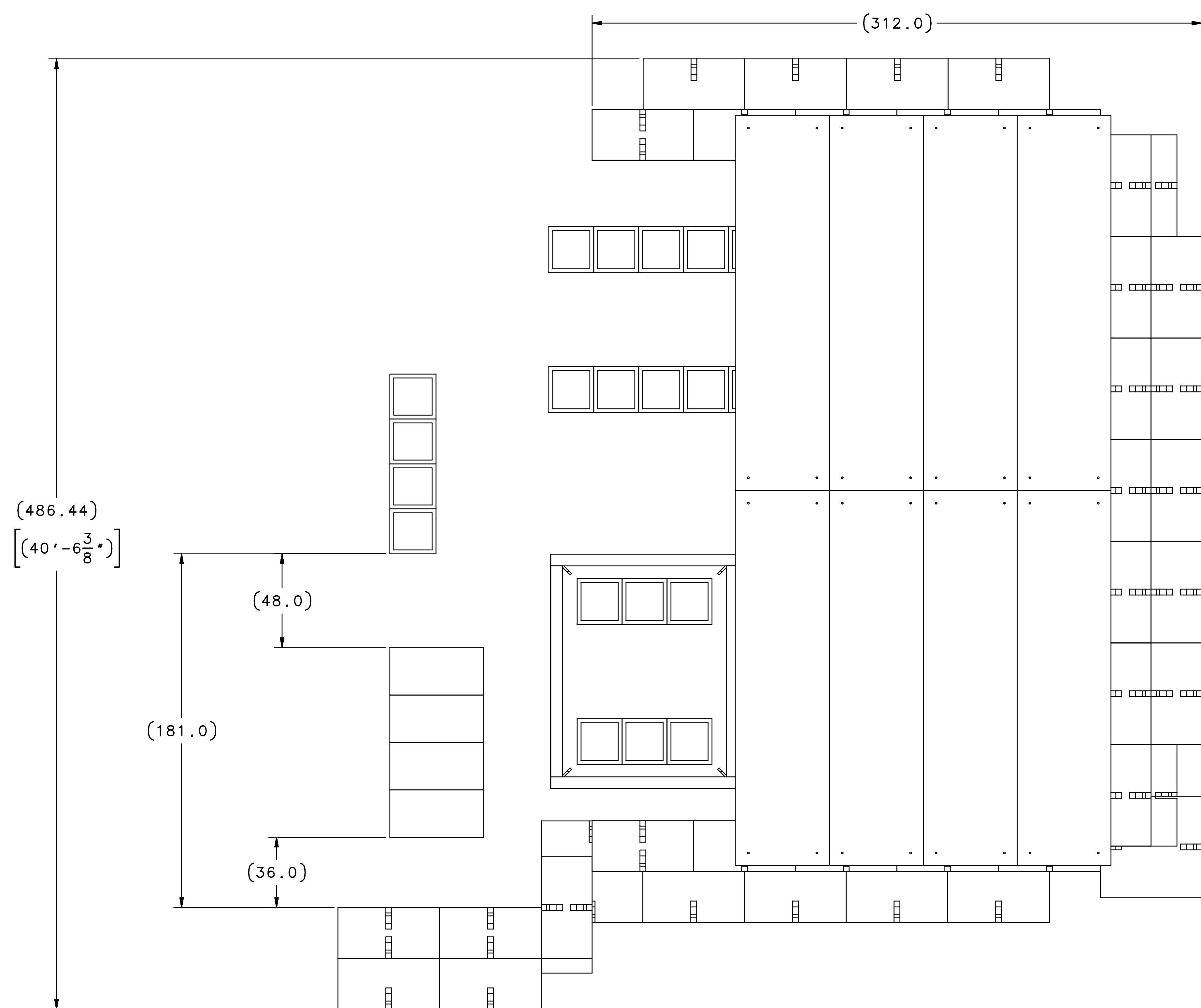
TOP VIEW
