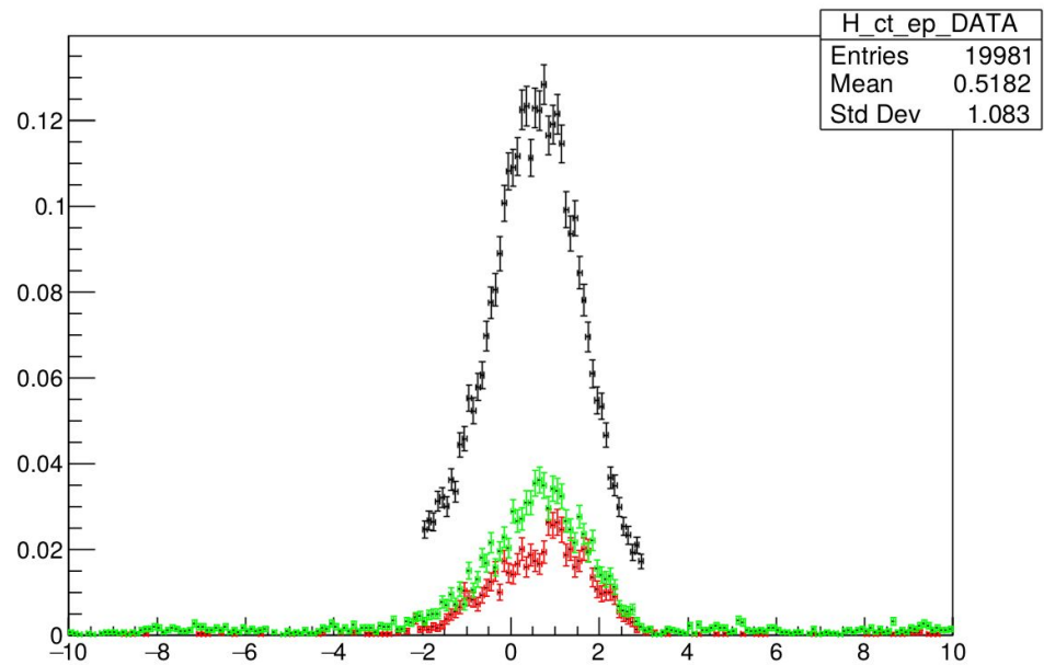
Electron-Proton CTime
