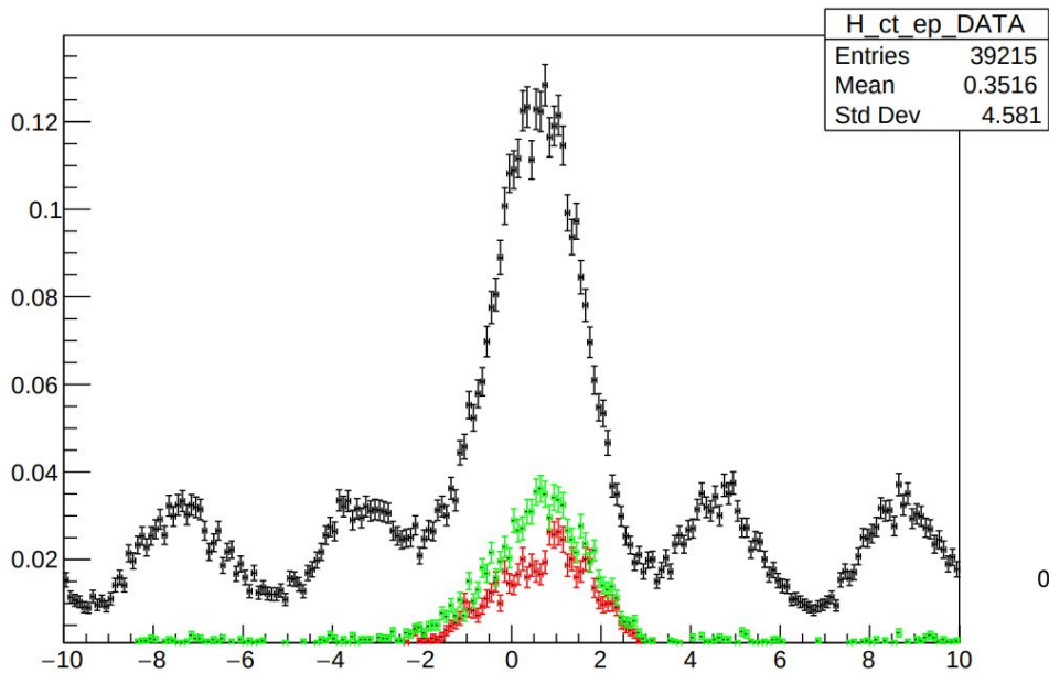
Electron-Proton CTime
