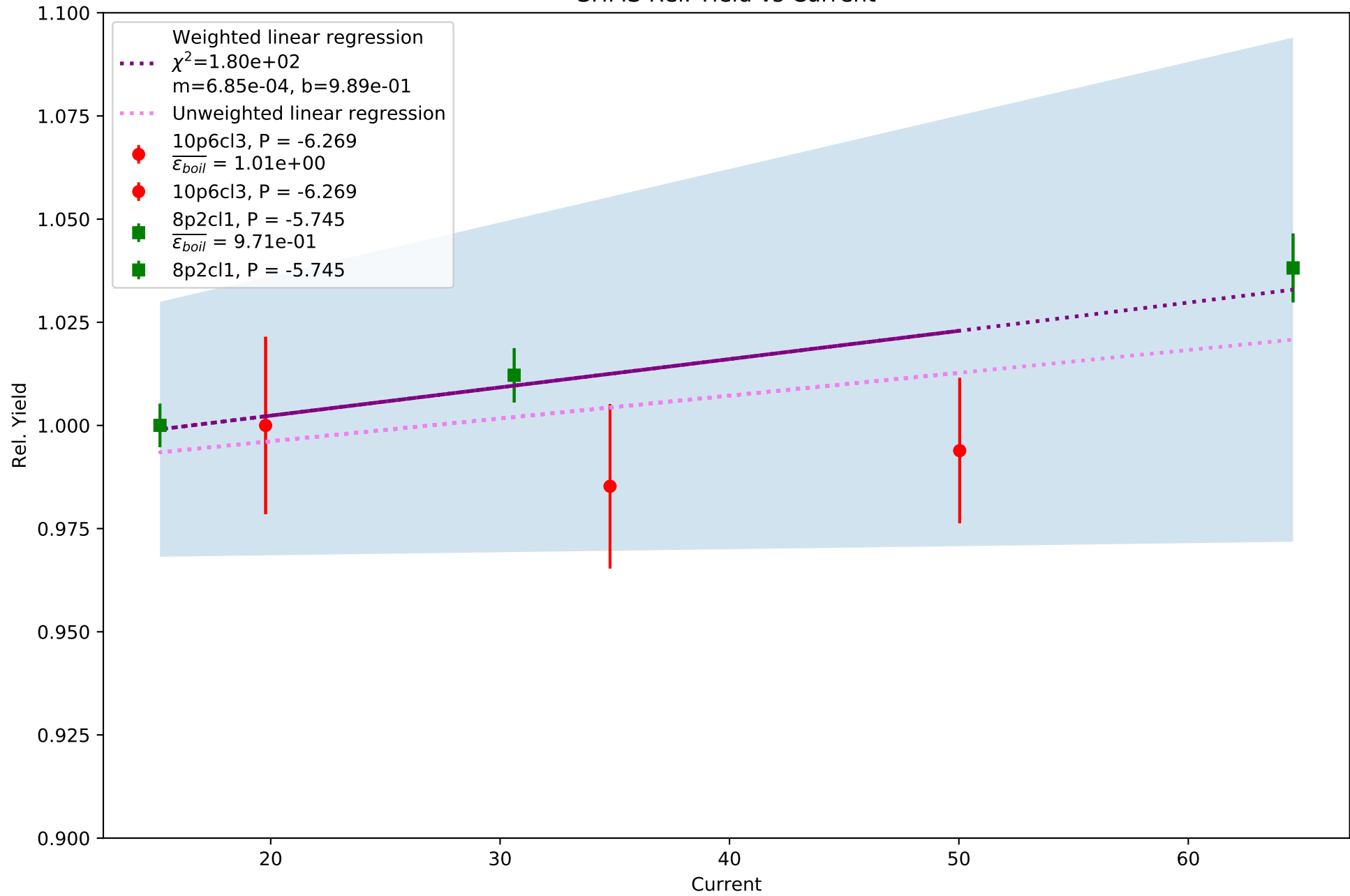
SHMS Rel. Yield vs Current
