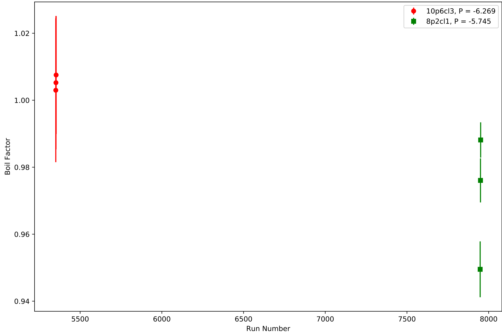
SHMS Boil Factor vs Run Number
