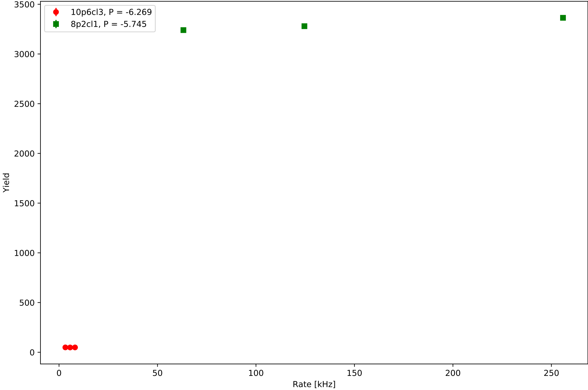
SHMS Yield vs Rate
