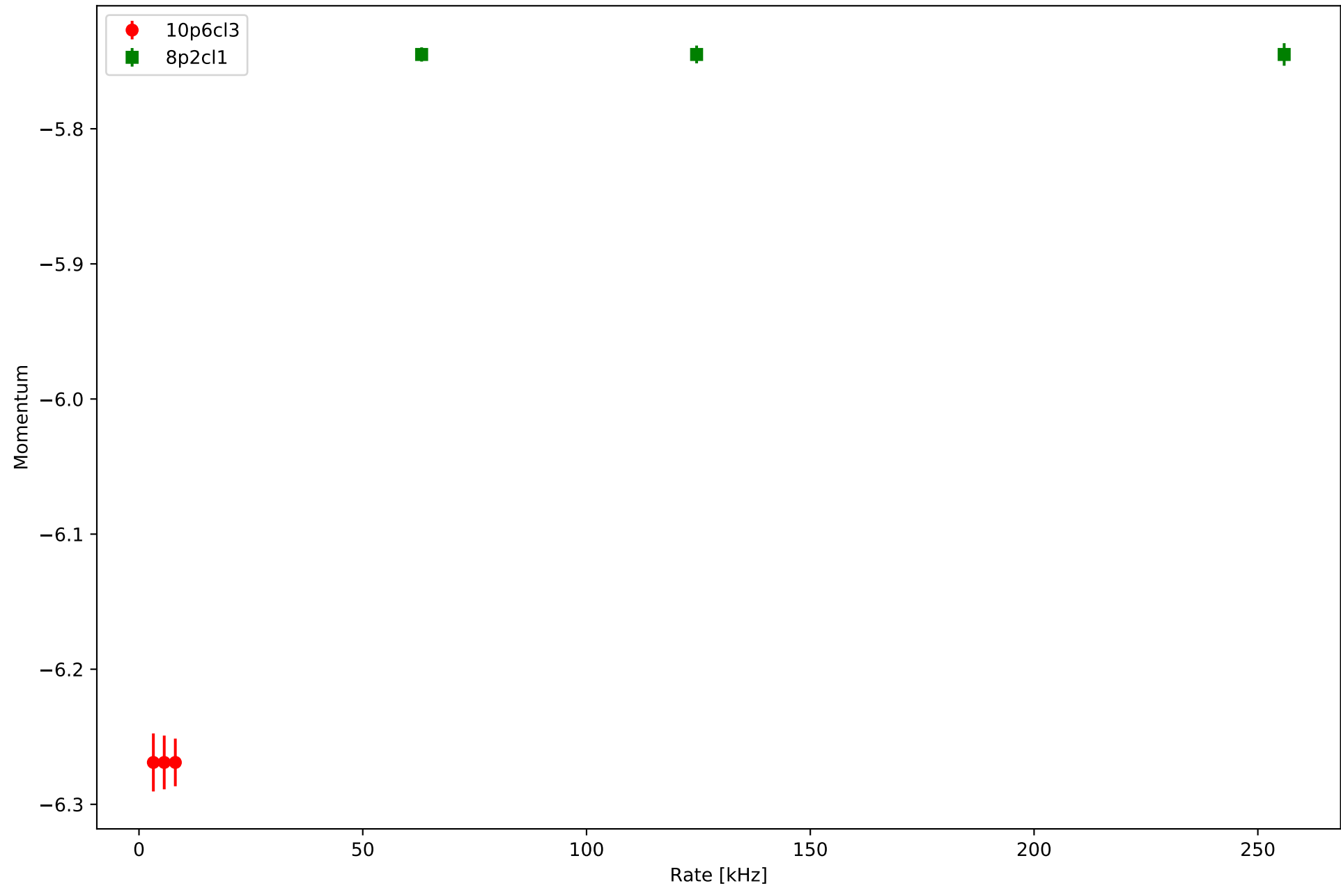
SHMS Momentum vs Rate
