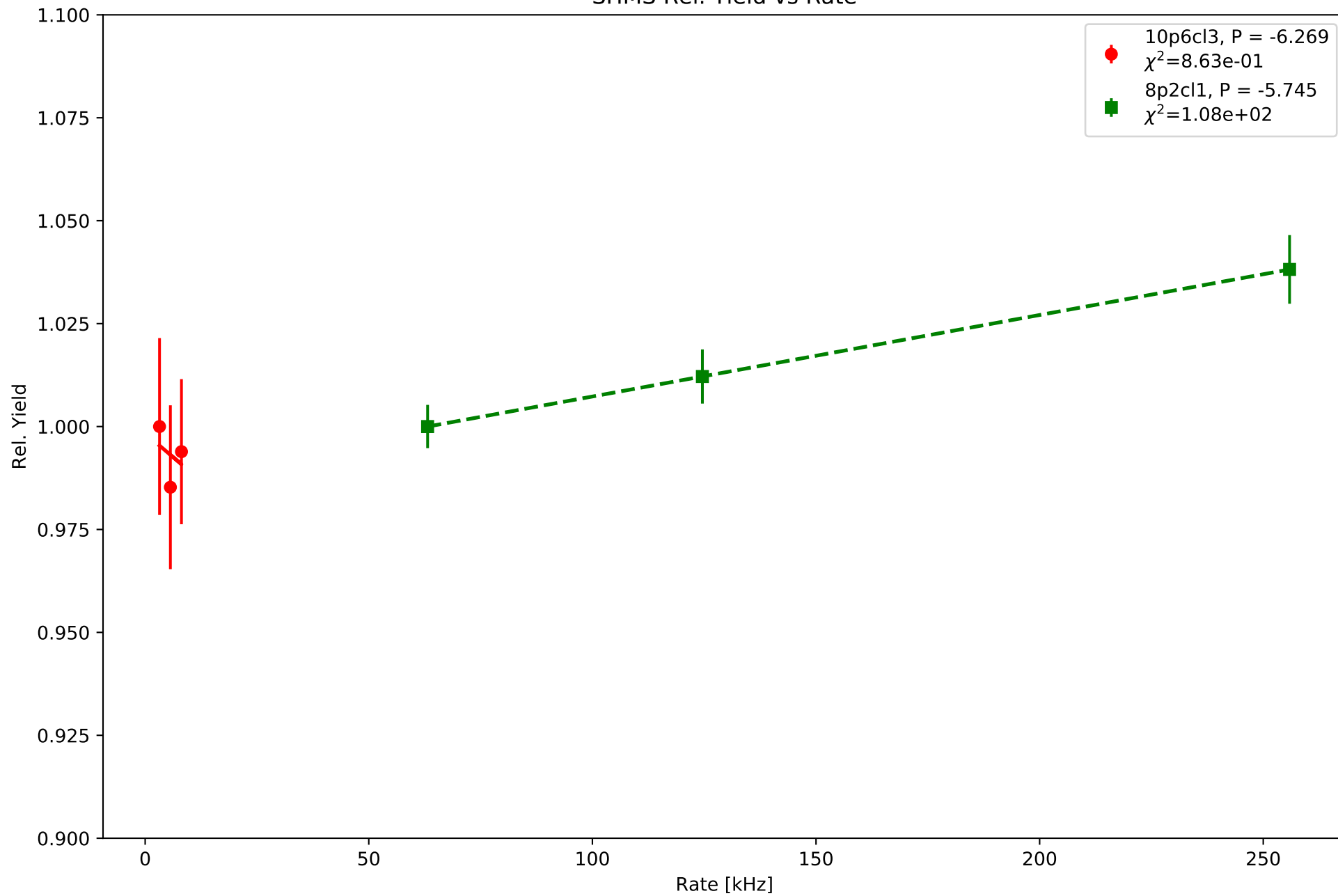
SHMS Rel. Yield vs Rate
