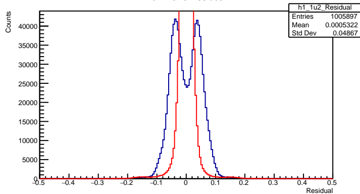
1u2 Plane Residual
