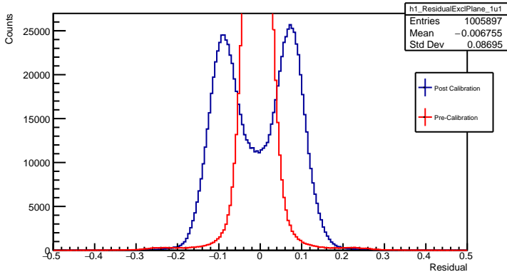
ResidualExcl Plane 1u1
