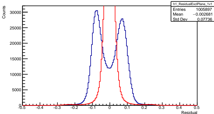
ResidualExcl Plane 1v1
