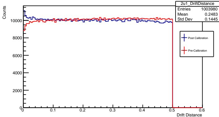
Drift Distance 2u1 Plane
