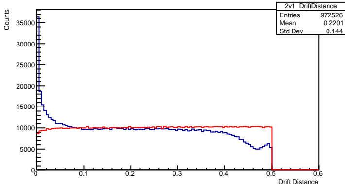
Drift Distance 2v1 Plane
