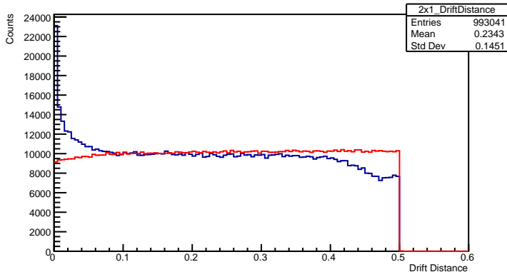
Drift Distance 2x1 Plane
