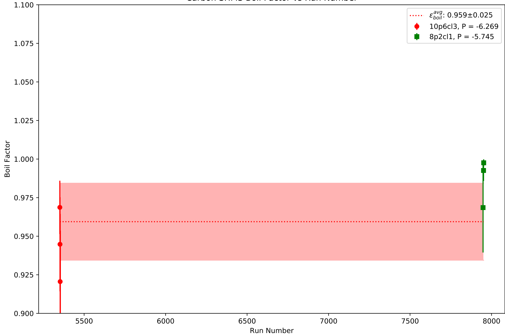
Carbon SHMS Boil Factor vs Run Number
