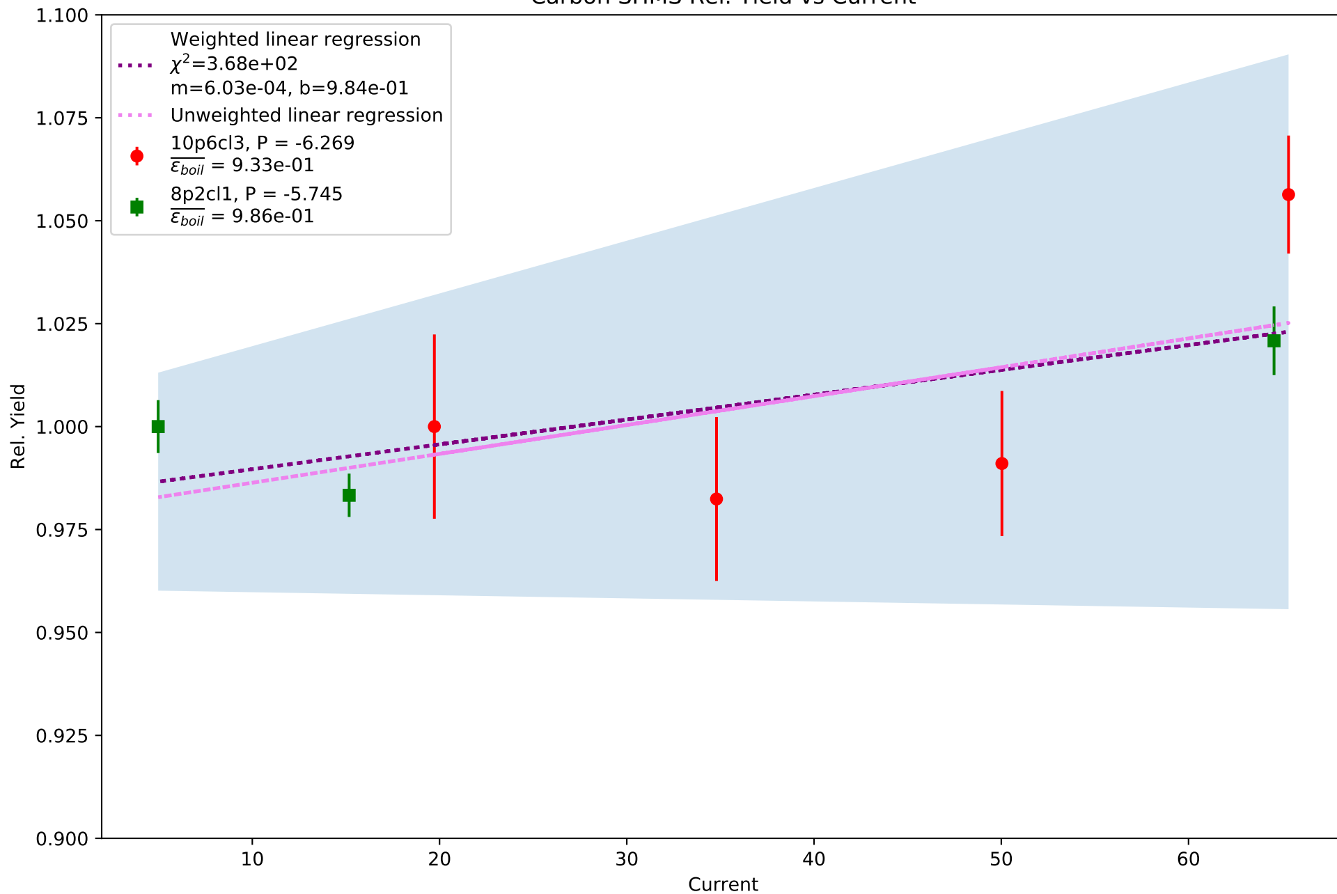
Carbon SHMS Rel. Yield vs Current
