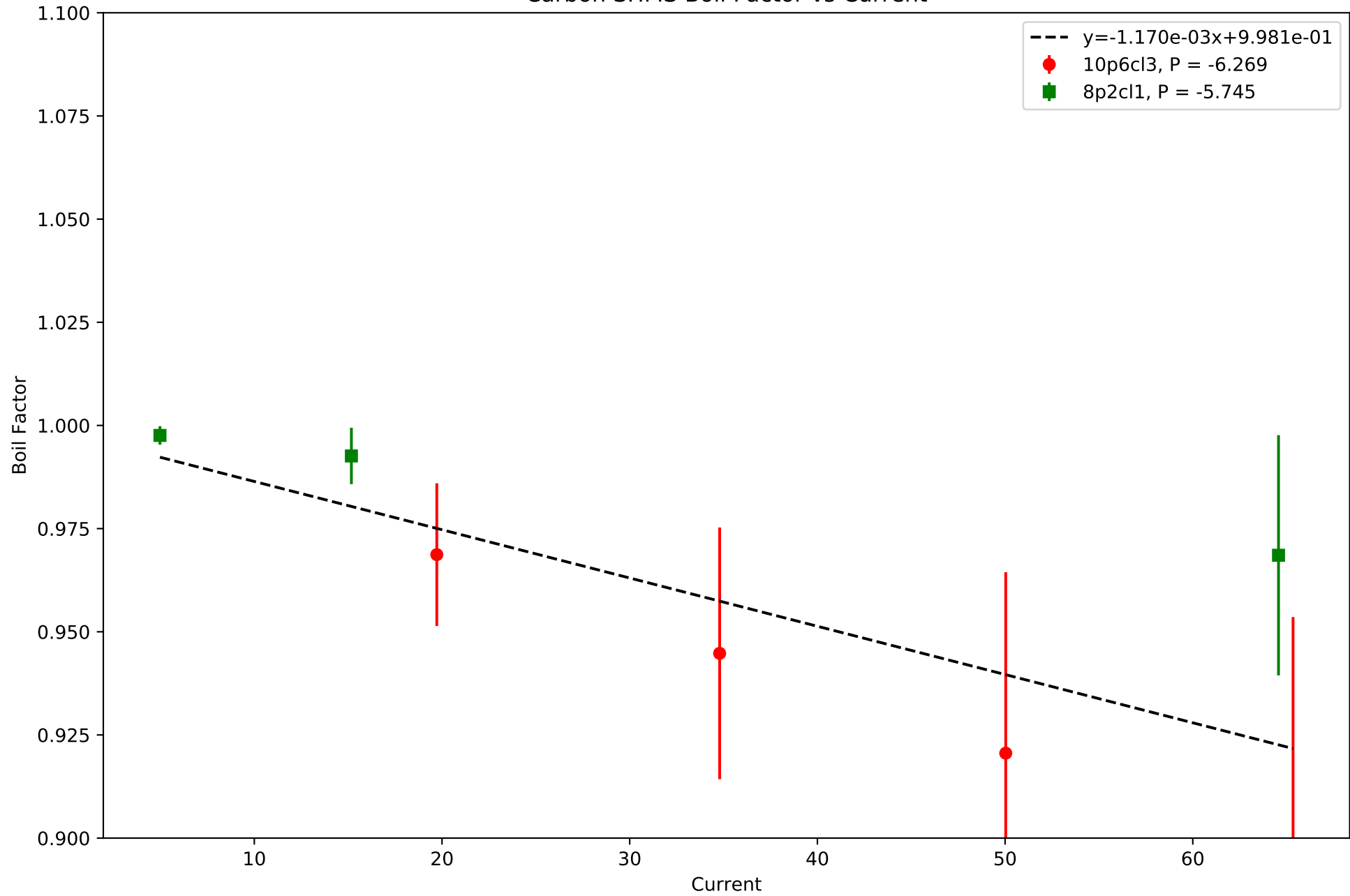
Carbon SHMS Boil Factor vs Current
