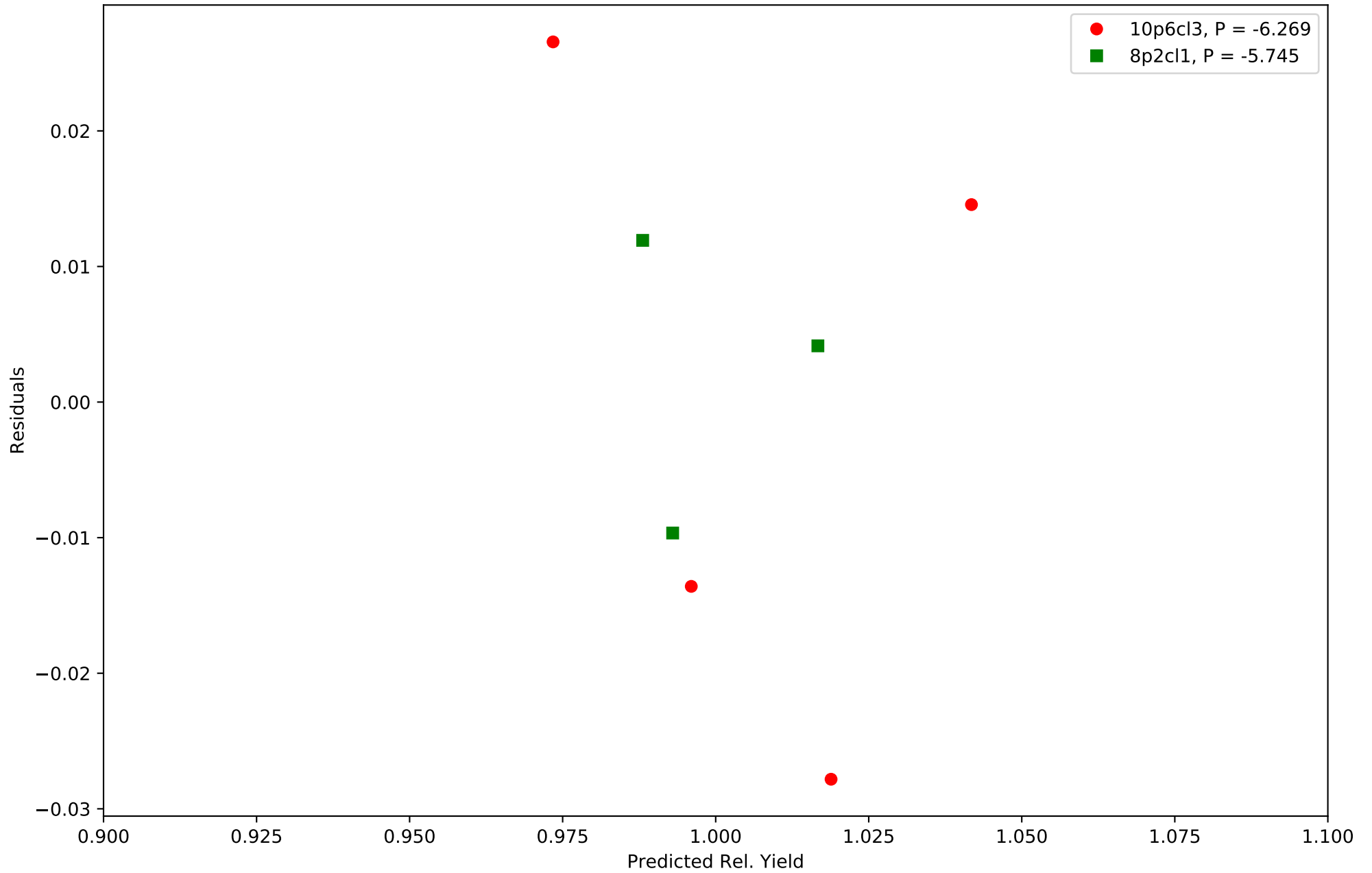
Residuals vs Predicted
