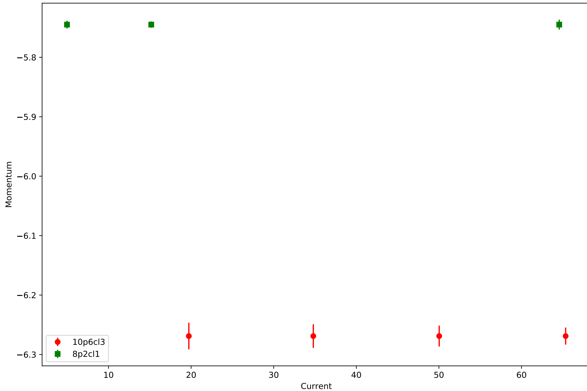
Carbon SHMS Momentum vs Current
