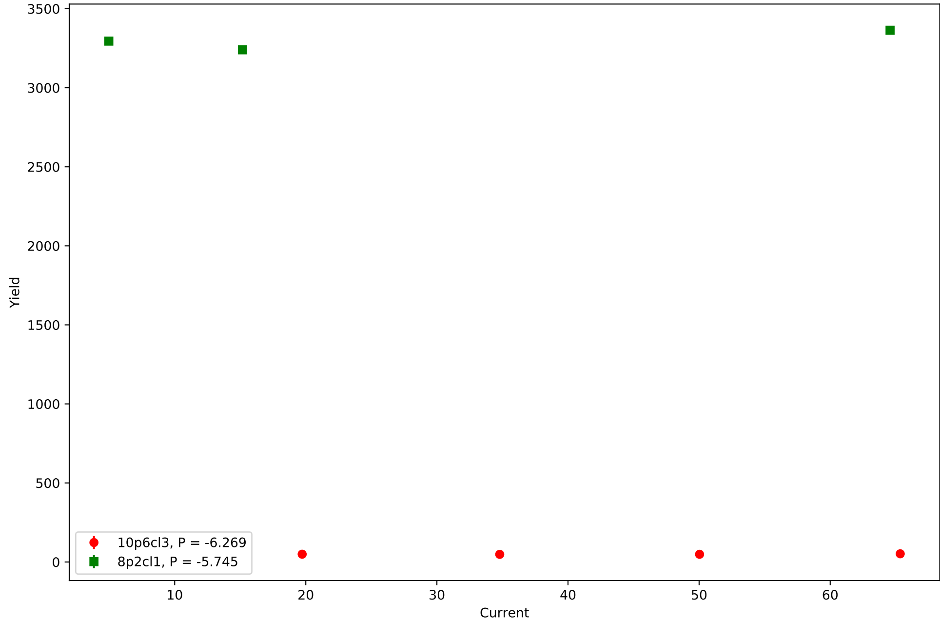
Carbon SHMS Yield vs Current
