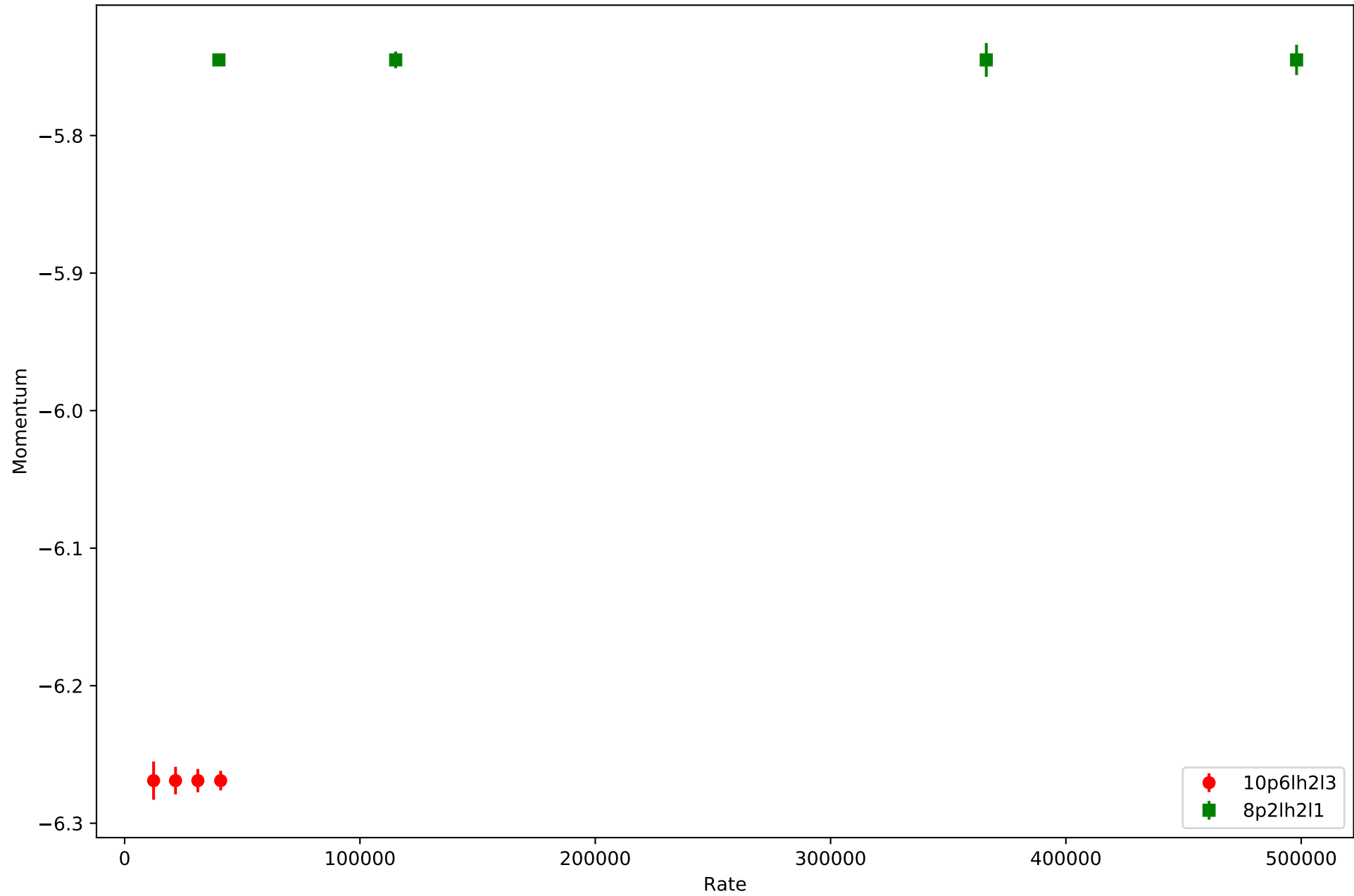
Lh2 SHMS Momentum vs Rate
