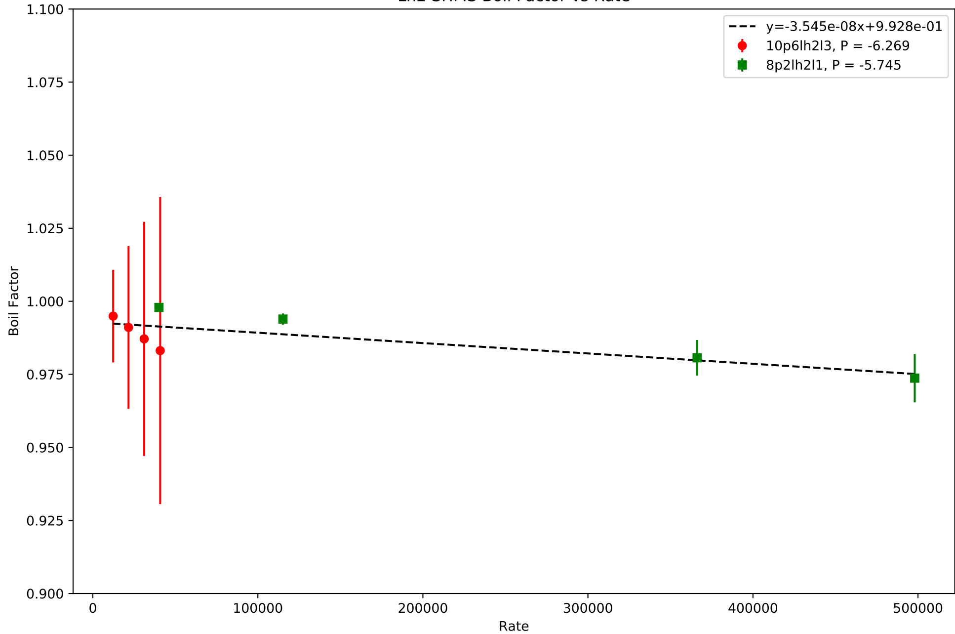
Lh2 SHMS Boil Factor vs Rate
