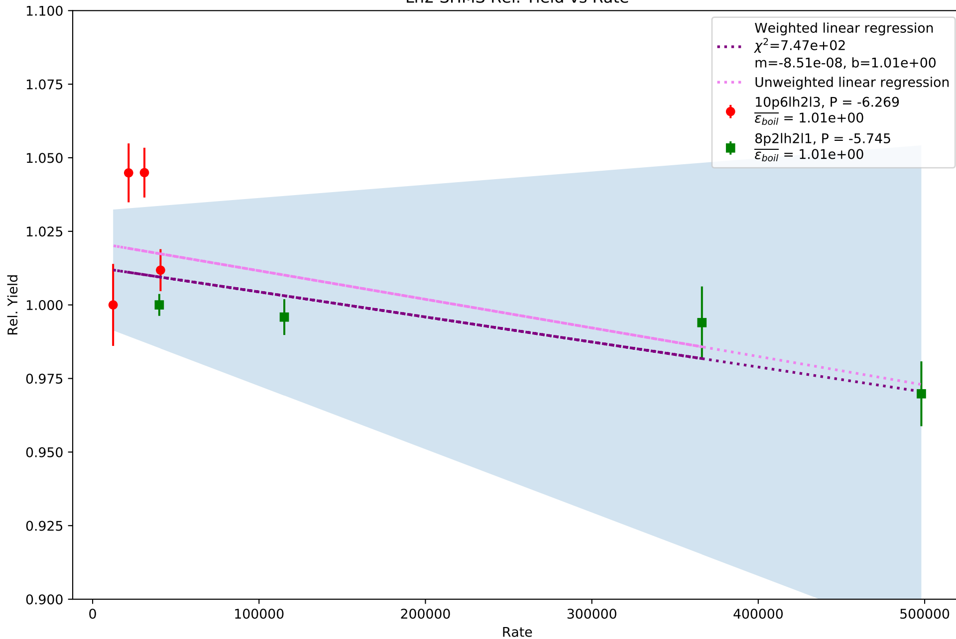
Lh2 SHMS Rel. Yield vs Rate
