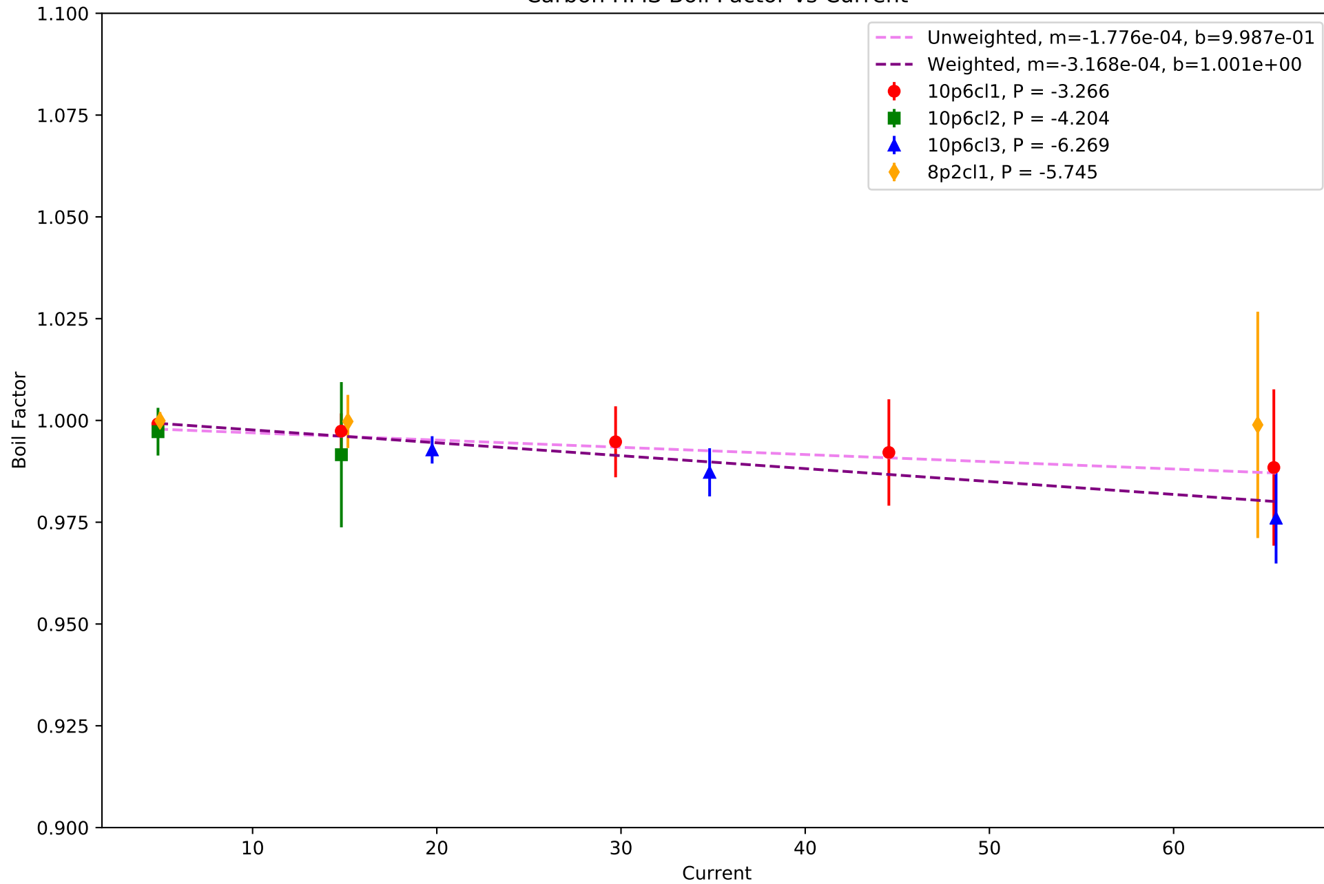
Carbon HMS Boil Factor vs Current
