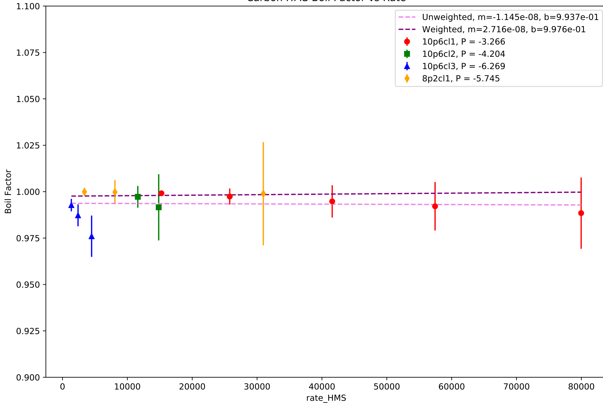
Carbon HMS Boil Factor vs Rate
