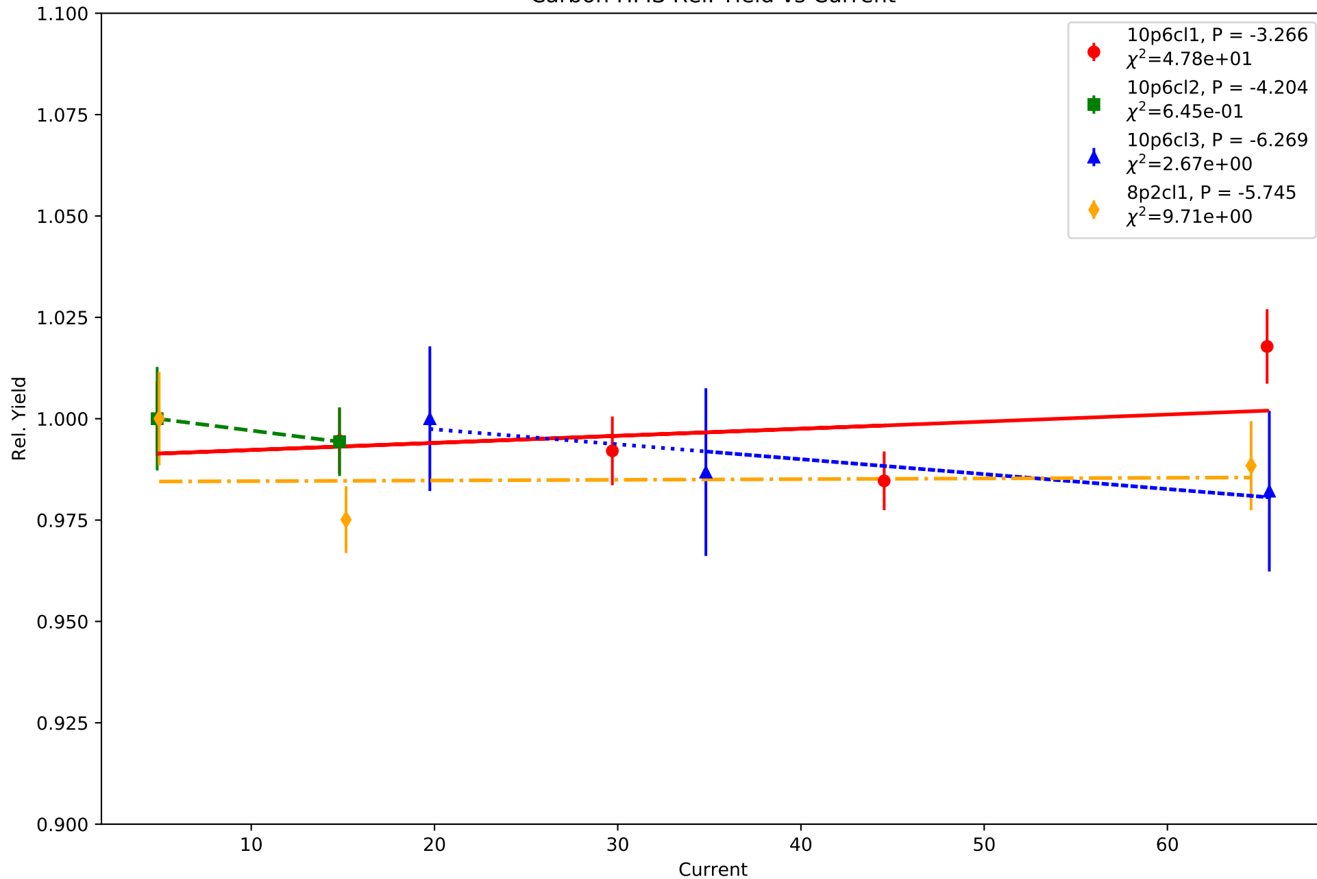
Carbon HMS Rel. Yield vs Current
