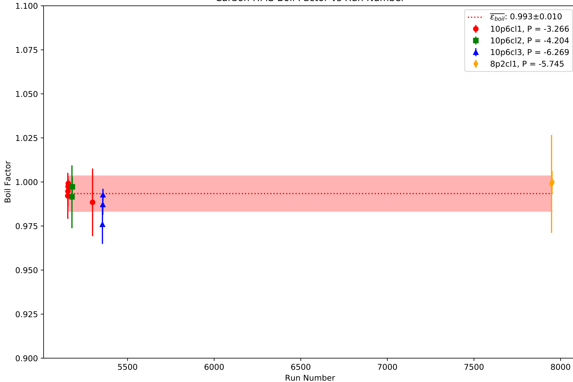
Carbon HMS Boil Factor vs Run Number
