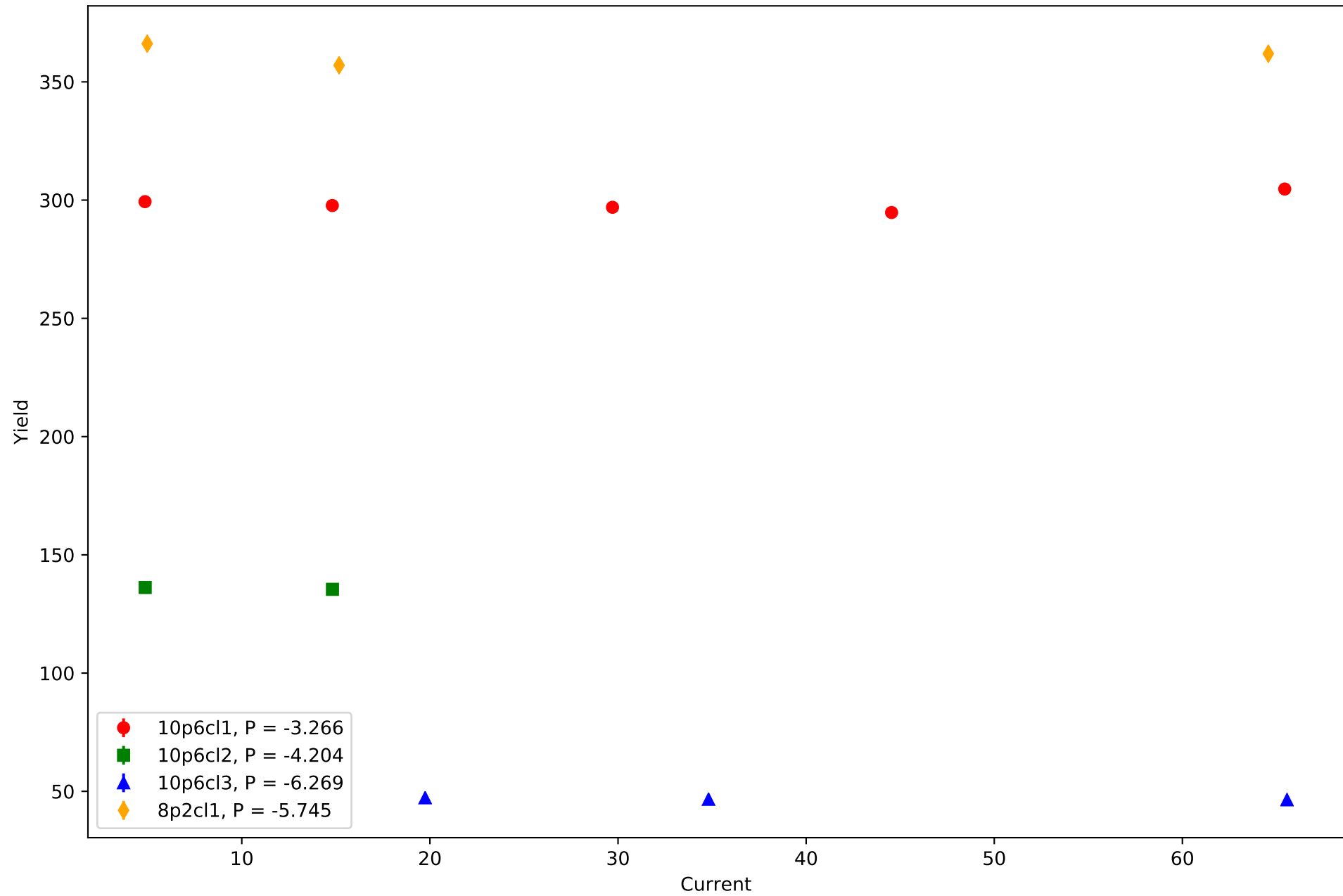
Carbon HMS Yield vs Current
