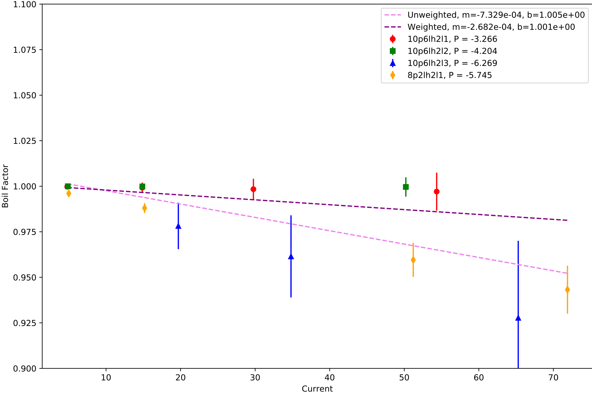
Lh2 HMS Boil Factor vs Current
