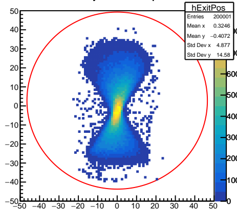
Tracks Projected to Dipole Exit
