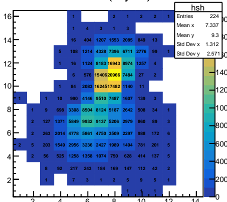
Shower (Layer2)
