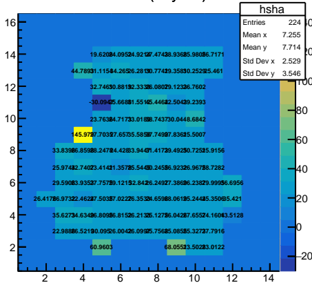
Shower (Layer2)
