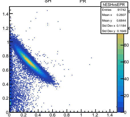
E_{\text{SH}} versus E_{\text{PR}}
