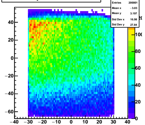
Tracks Projected to Calorimeter
