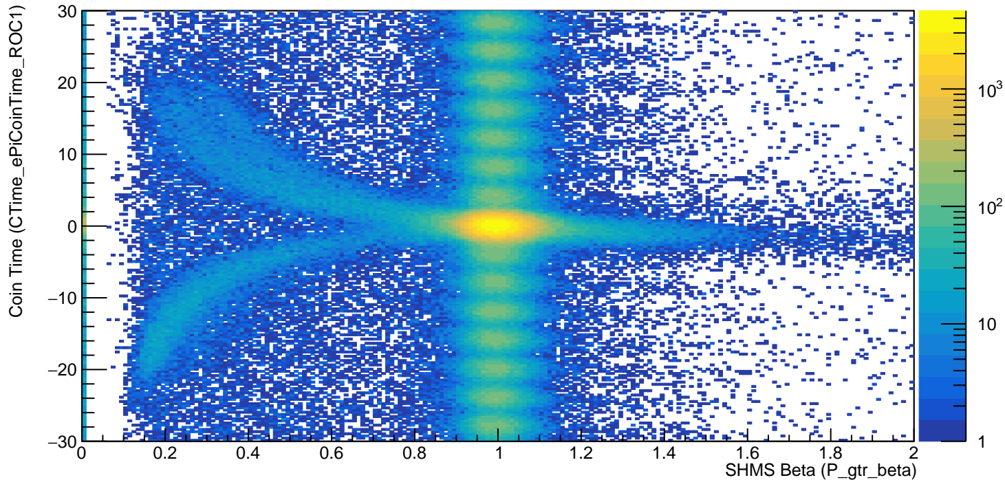
Coin Time vs SHMS Beta (pi-N)
