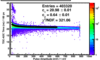
TDC-ADC Time vs. Pulse Amp Plane 2y Side pos Paddle 5
