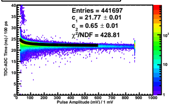
TDC-ADC Time vs. Pulse Amp Plane 2y Side pos Paddle 6
