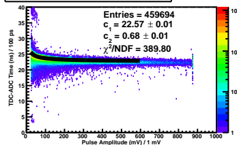
TDC-ADC Time vs. Pulse Amp Plane 2y Side pos Paddle 7
