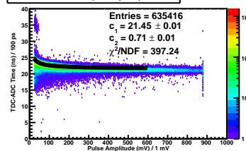
TDC-ADC Time vs. Pulse Amp Plane 2y Side pos Paddle 8
