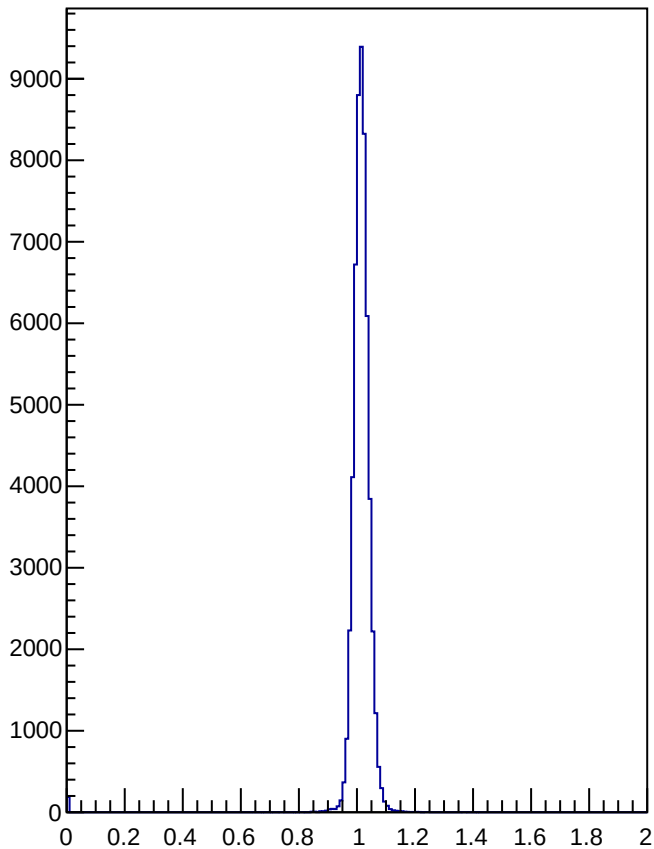
HMS_β no cut
