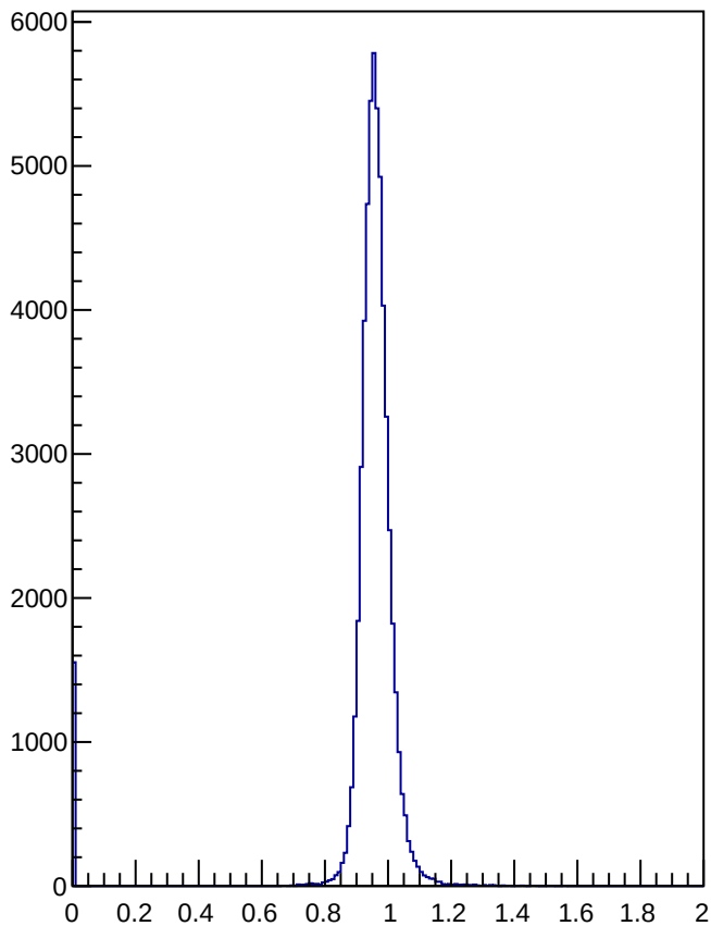
SHMS_ \beta no cut
