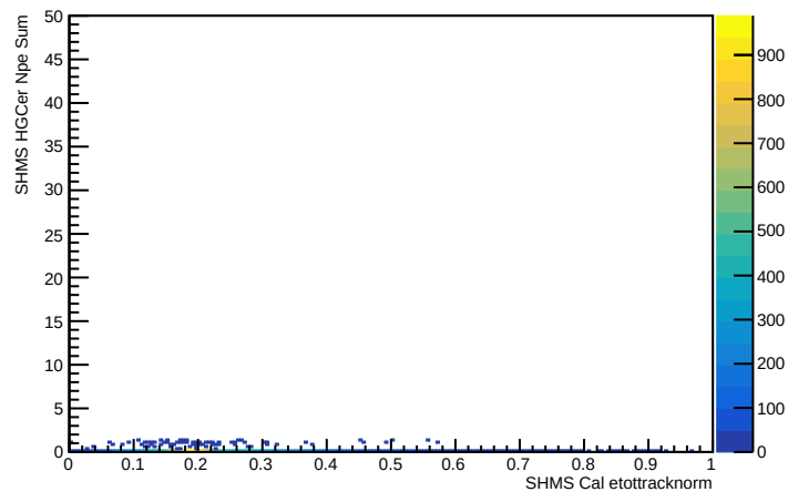
SHMS Cal etottracknorm vs SHMS HGCer Npe Sum
