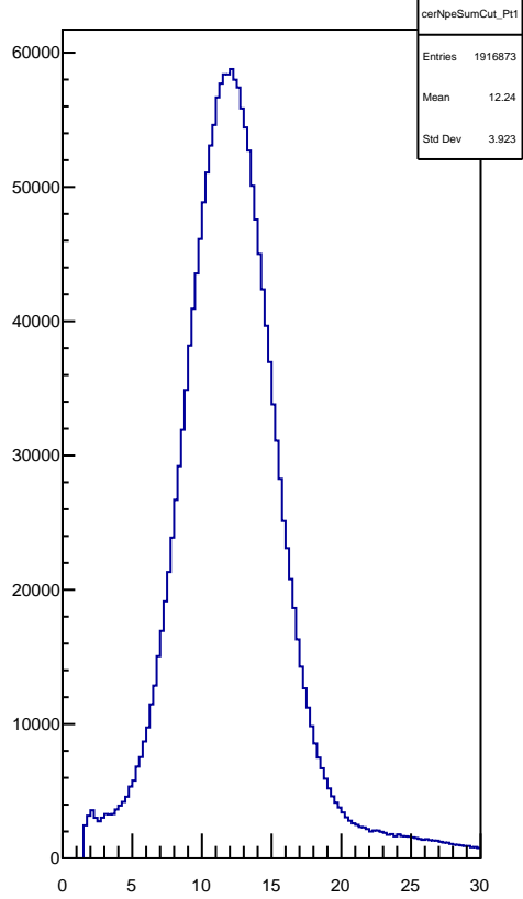
cerNpeSumCut_Pt1
