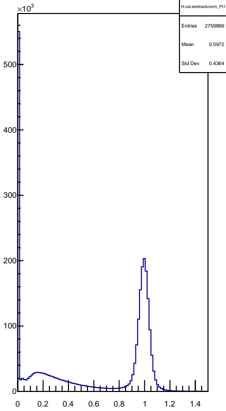
H.cal.etottracknorm_Pt1
