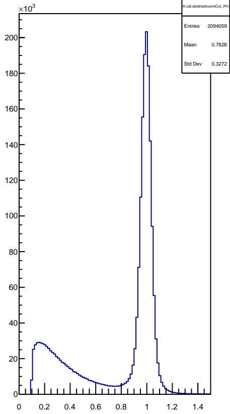
H.cal.etottracknormCut_Pt1
