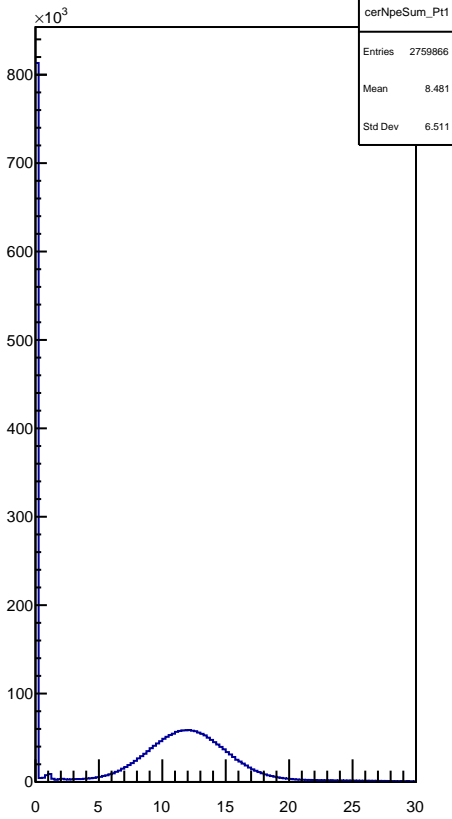
cerNpeSum_Pt1
