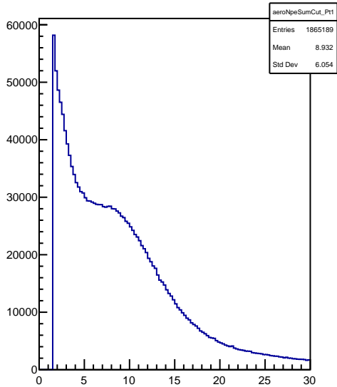
aeroNpeSumCut_Pt1
