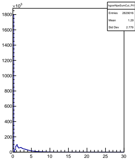
hgcerNpeSumCut_Pt1
