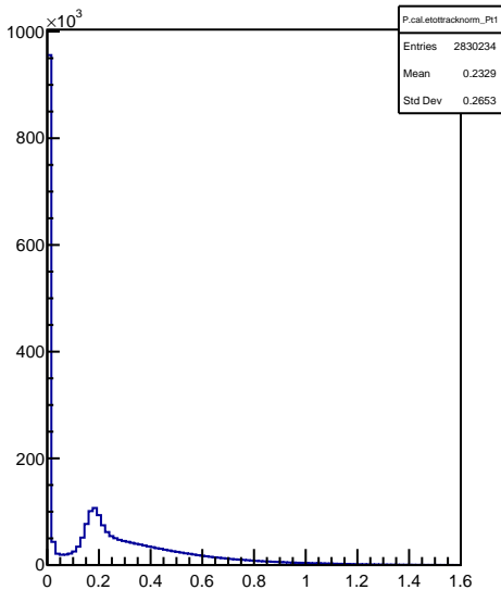
P.cal.etottracknorm_Pt1
