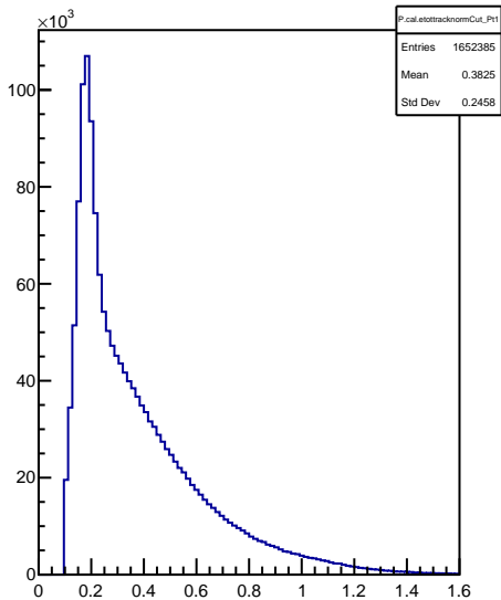
P.cal.etottracknormCut_Pt1
