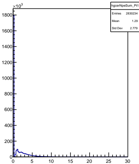
hgcerNpeSum_Pt1
