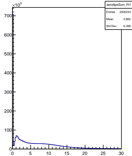
aeroNpeSum_Pt1
