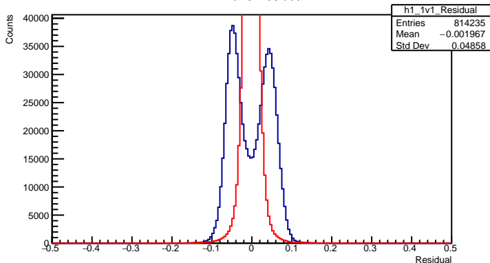
1v1 Plane Residual
