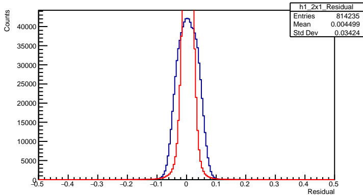
2x1 Plane Residual
