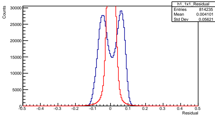
1x1 Plane Residual
