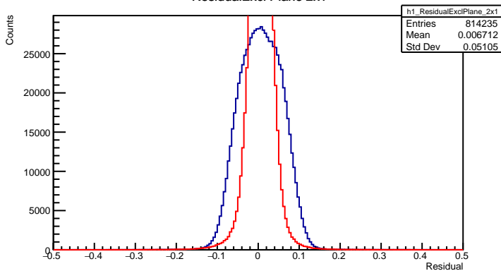
ResidualExcl Plane 2x1
