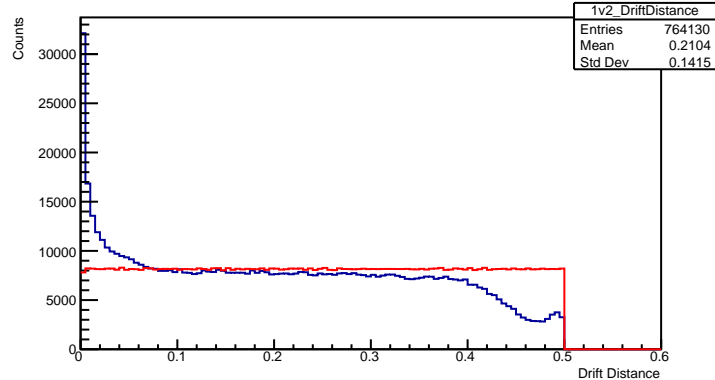
Drift Distance 1v2 Plane
