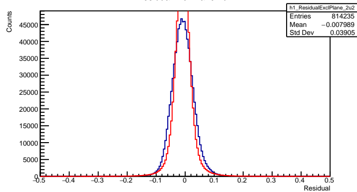
ResidualExcl Plane 2u2
