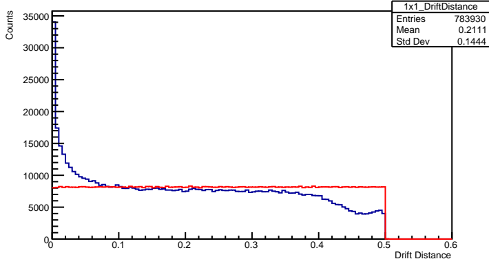
Drift Distance 1x1 Plane
