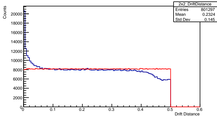
Drift Distance 2x2 Plane
