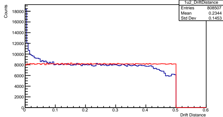
Drift Distance 1u2 Plane
