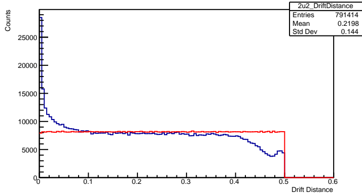
Drift Distance 2u2 Plane
