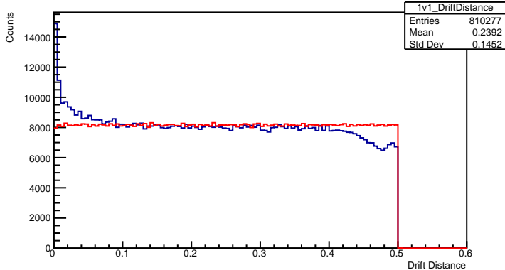
Drift Distance 1v1 Plane
