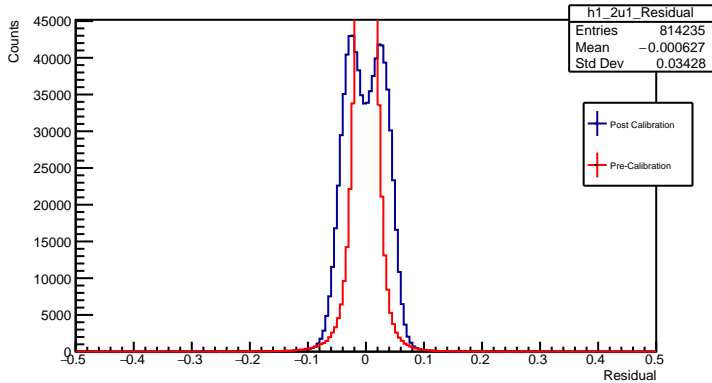
2u1 Plane Residual
