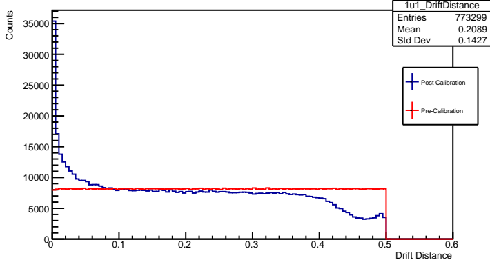
Drift Distance 1u1 Plane
