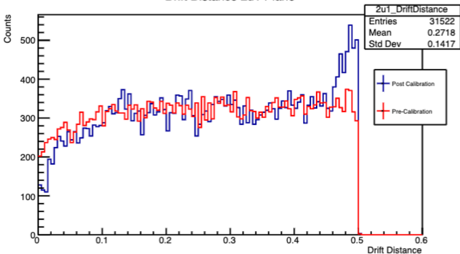
Drift Distance 2u1 Plane
