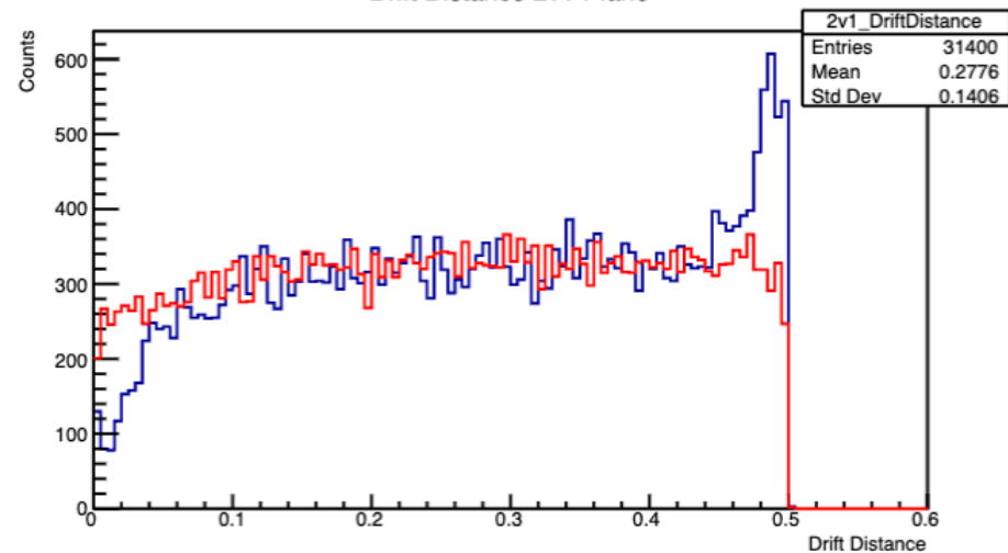
Drift Distance 2v1 Plane
