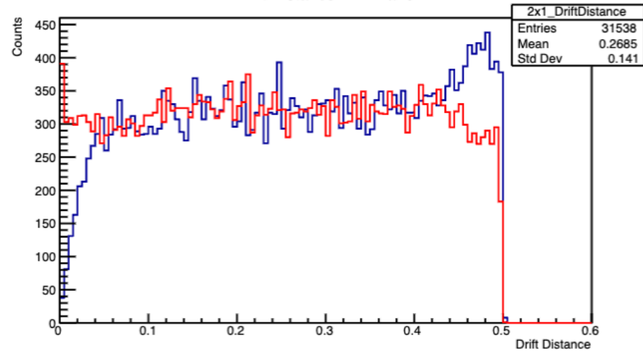
Drift Distance 2x1 Plane
