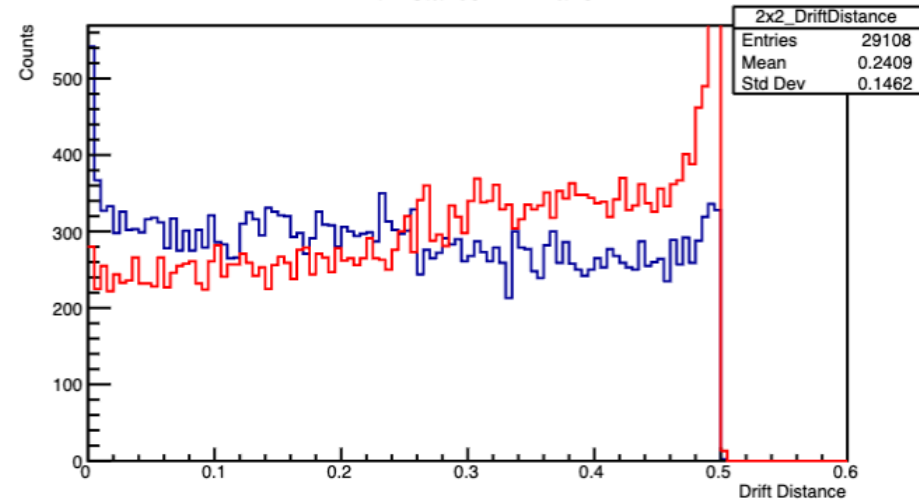
Drift Distance 2x2 Plane
