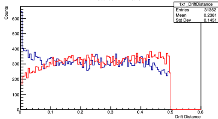
Drift Distance 1x1 Plane
