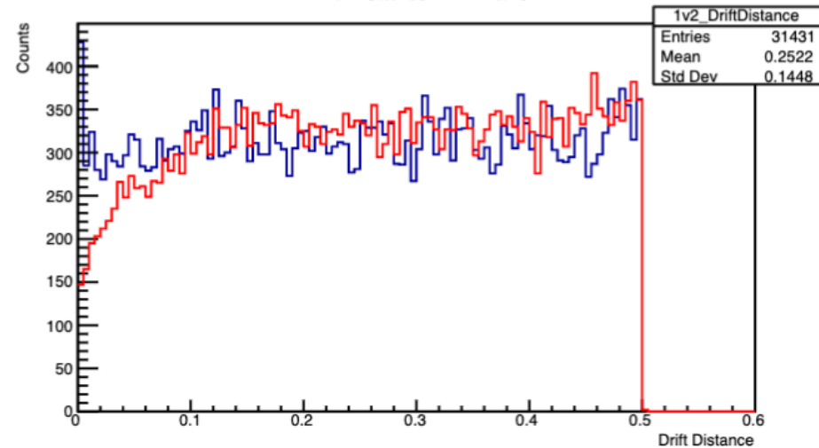
Drift Distance 1v2 Plane
