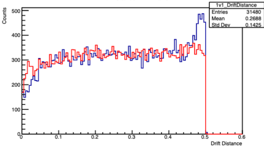
Drift Distance 1v1 Plane
