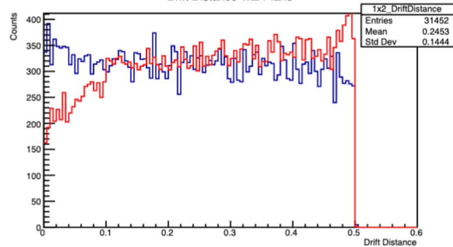
Drift Distance 1x2 Plane
