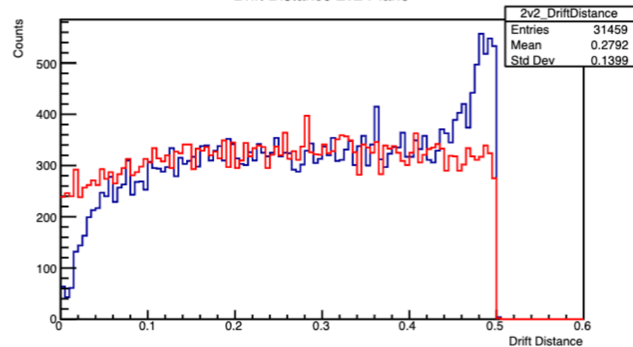
Drift Distance 2v2 Plane
