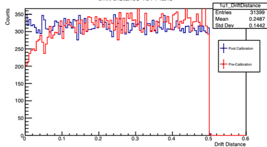
Drift Distance 1u1 Plane
