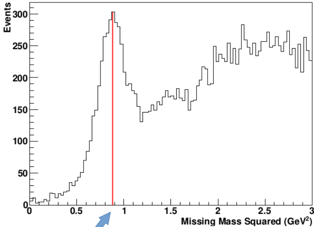
Missing Mass Squared ( \text{GeV}^2 )
