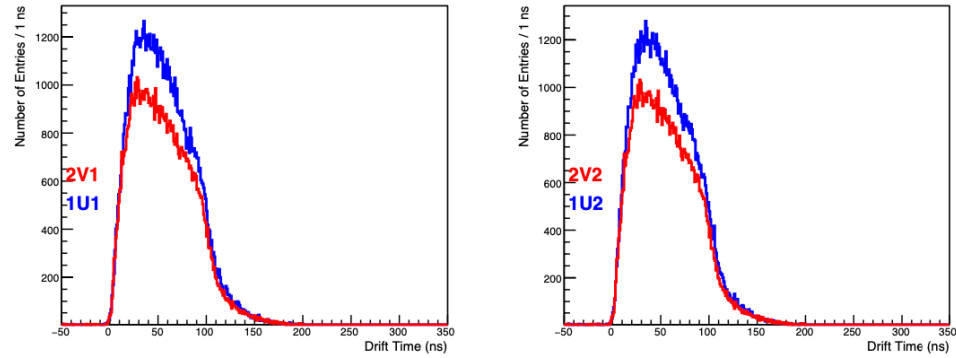
Summary Plots(Run #3991): HMS Drift Chamber Drift Time
