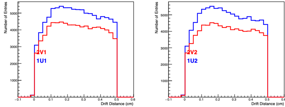
Summary Plots(Run #3991): HMS Drift Chamber Drift Distance
