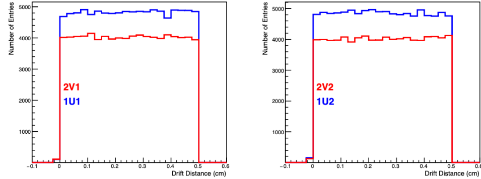
Summary Plots(Run #3991): HMS Drift Chamber Drift Distance
