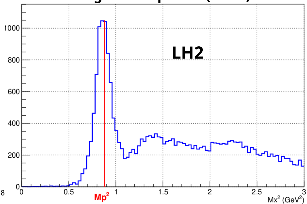
Missing Mass Squared (GeV 2 )
