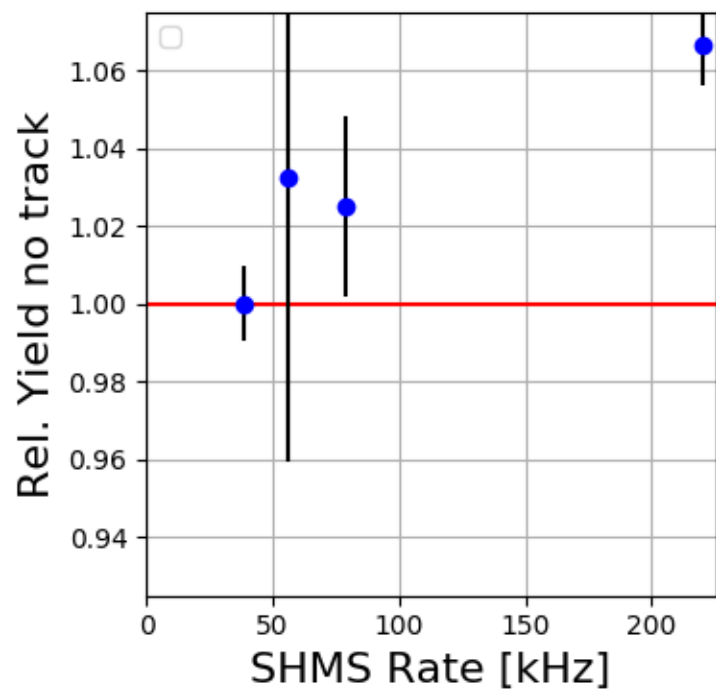
SHMS Carbon 12144-12151
