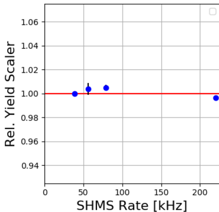
SHMS Carbon 12144-12151
