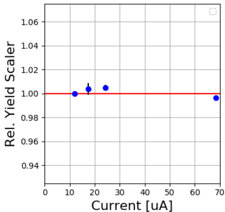
SHMS Carbon 12144-12151
