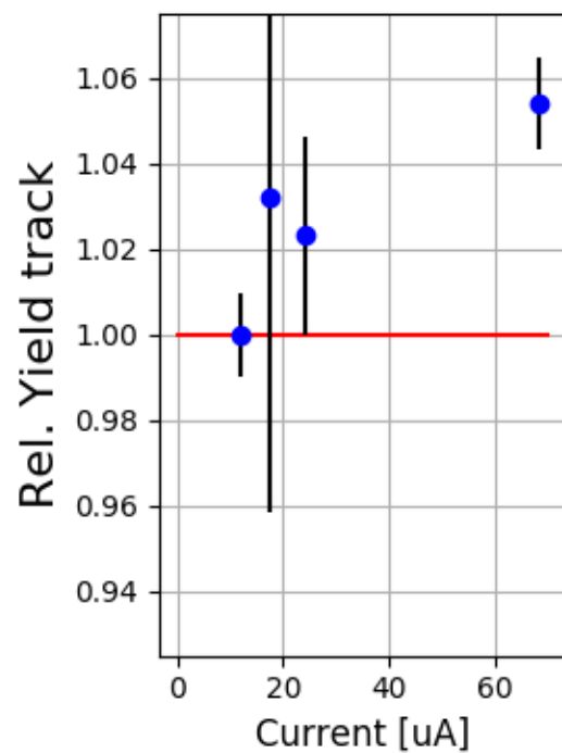
SHMS Carbon 12144-12151
