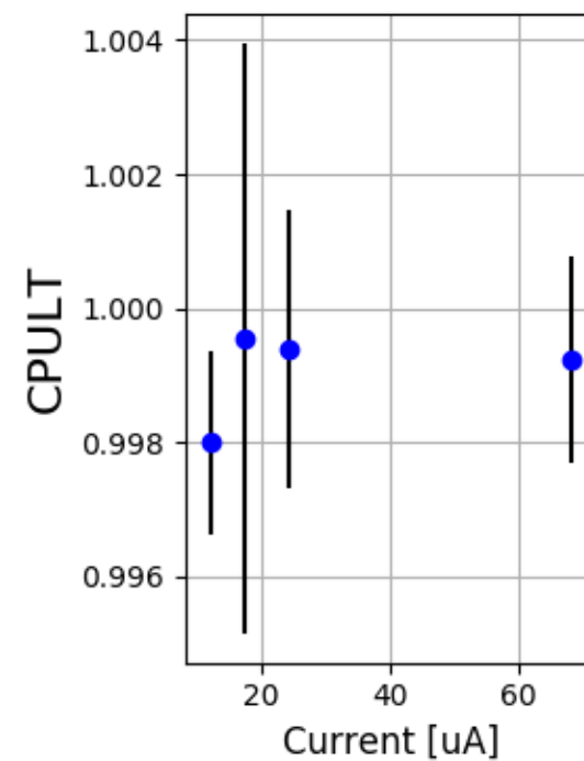
Carbon 12144-12151
