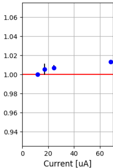
SHMS Carbon 12144-12151
