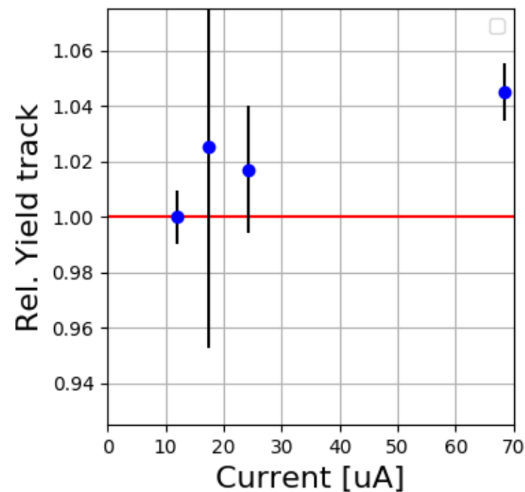
SHMS Carbon 12144-12151
