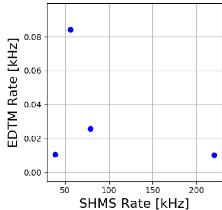
SHMS Carbon 12144-12151
