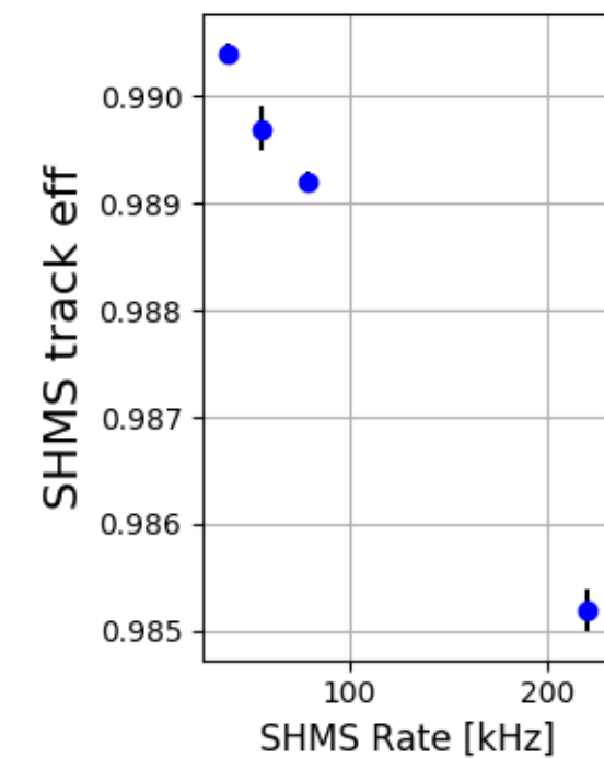
SHMS Carbon 12144-12151
