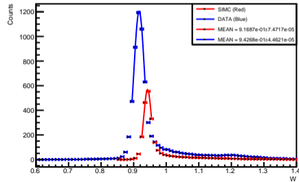
W Distribution
