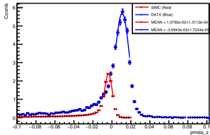
Momentum_z Distribution
