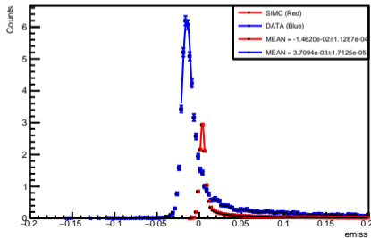
Energy Distribution
