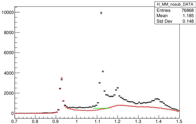
MM_nosub K
