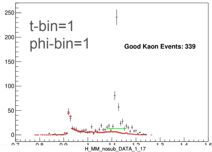
H_MM_nosub_DATA_0_0
