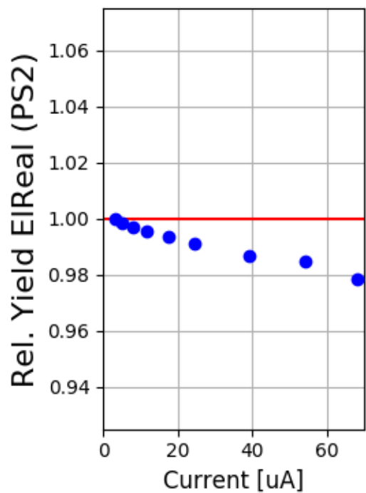
SHMS Carbon 12144-12154
