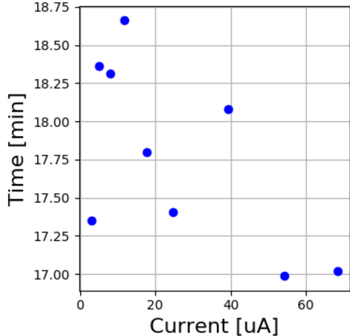
HMS Carbon 12144-12154
