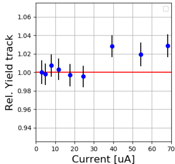
SHMS Carbon 12144-12154
