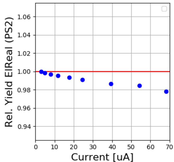
SHMS Carbon 12144-12154
