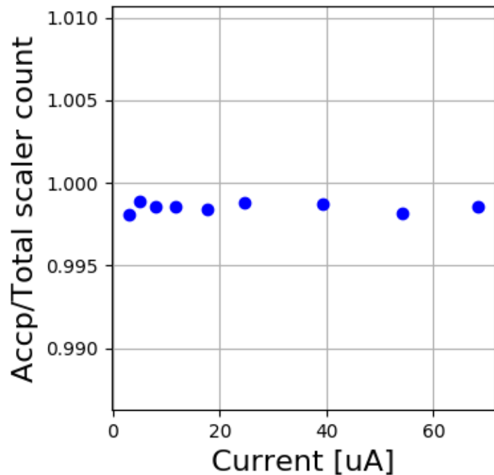
Carbon 12144-12154
