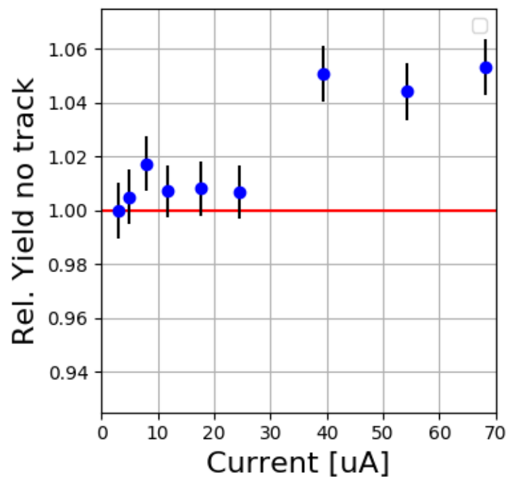
SHMS Carbon 12144-12154
