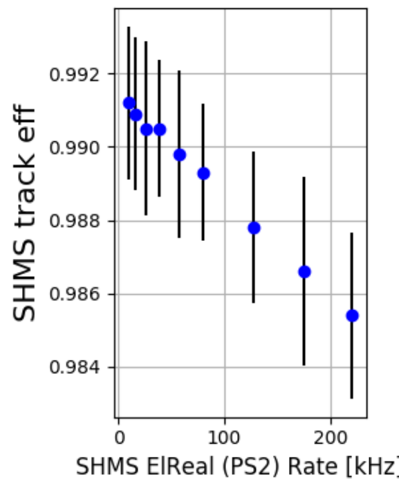
SHMS Carbon 12144-12154
