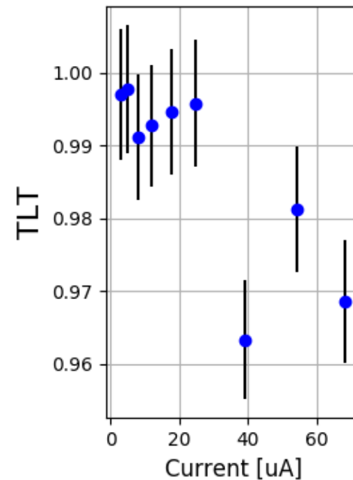
Carbon 12144-12154
