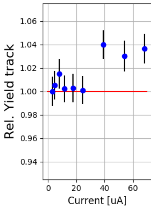
SHMS Carbon 12144-12154
