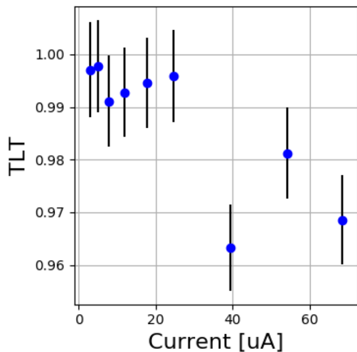
Carbon 12144-12154
