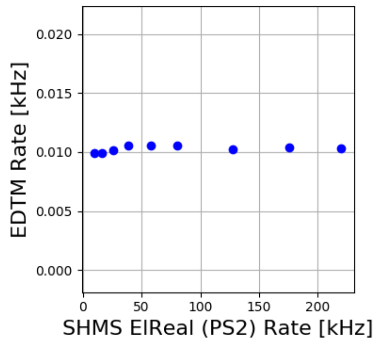
SHMS Carbon 12144-12154
