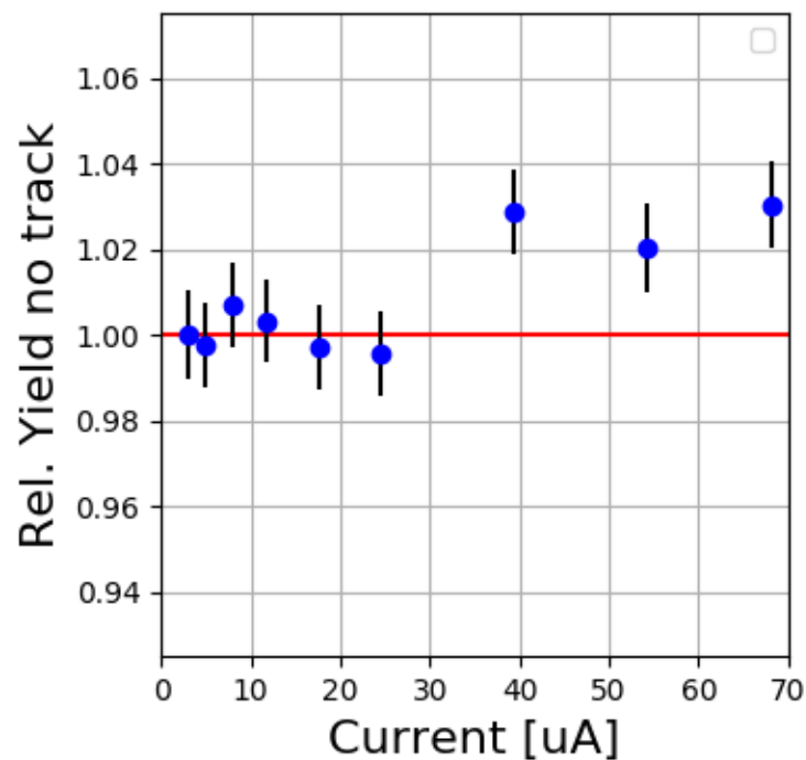
SHMS Carbon 12144-12154
