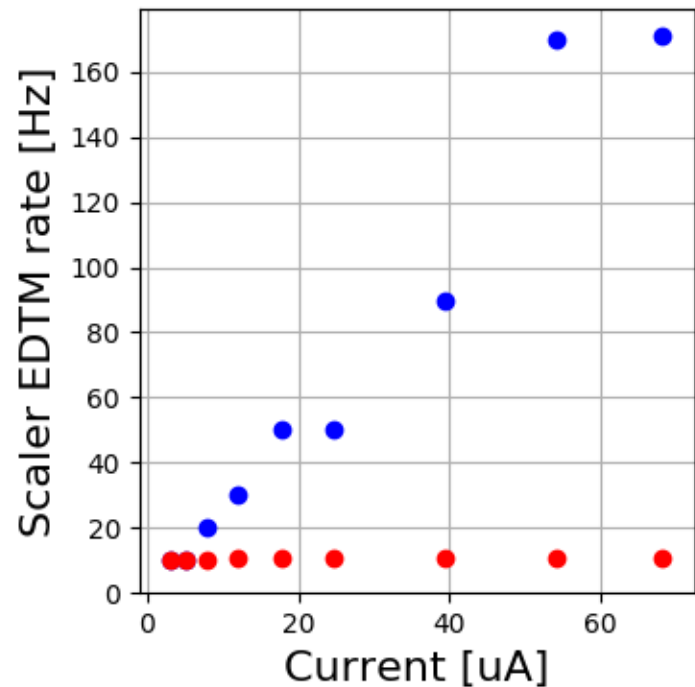
HMS Carbon 12144-12154
