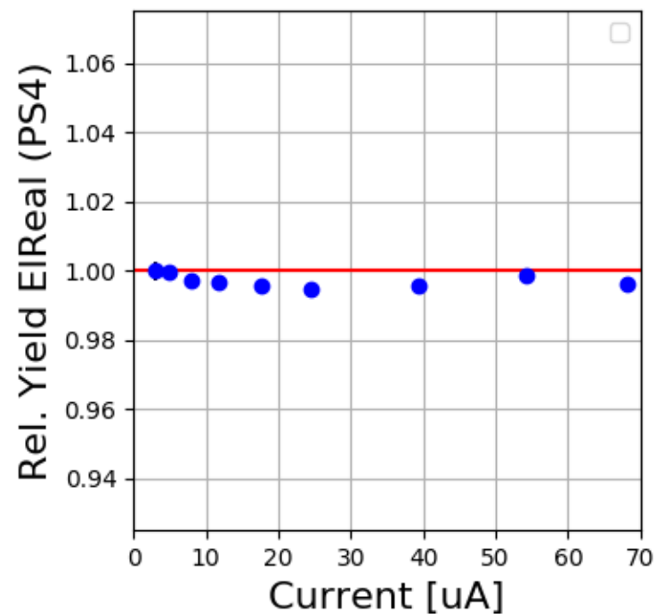
SHMS Carbon 12144-12154
