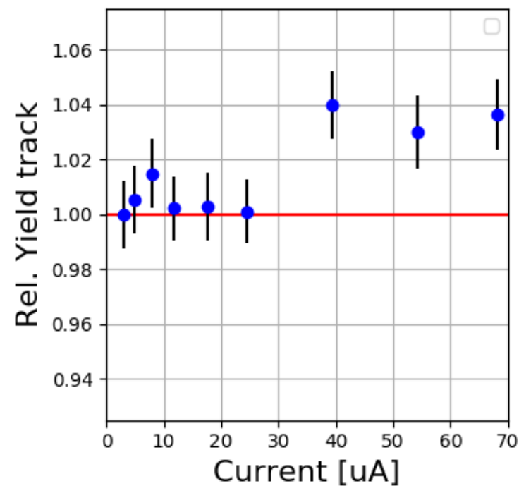
SHMS Carbon 12144-12154
