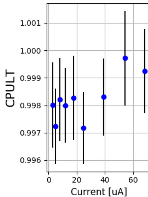
Carbon 12144-12154
