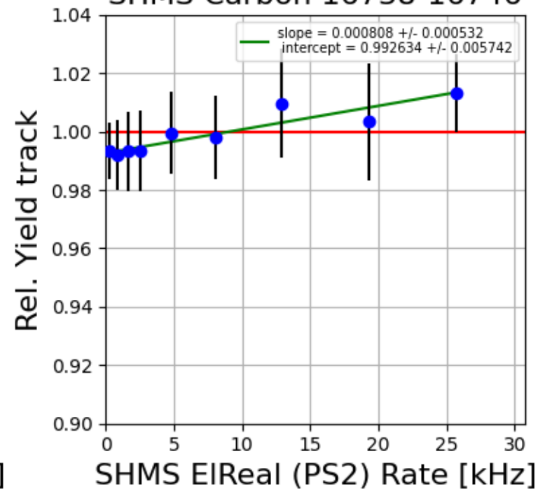
SHMS Carbon 16738-16746
