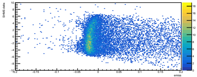
emiss vs SHMS delta
