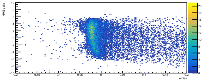
emiss vs HMS delta
