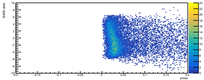
pmiss vs SHMS delta
