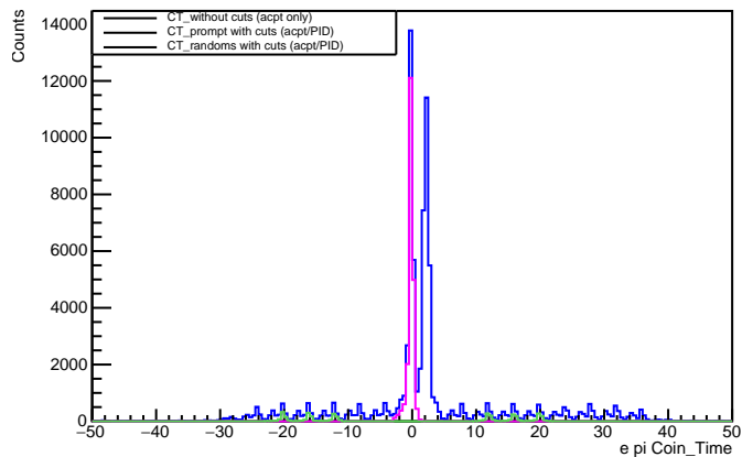
Electron-Pion CTime (acpt_cut)
