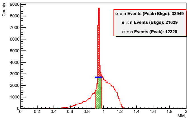
Missing Mass data (accpt_cut)
