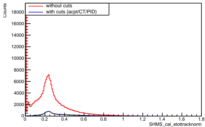
SHMS cal etotracknorm (uncut)
