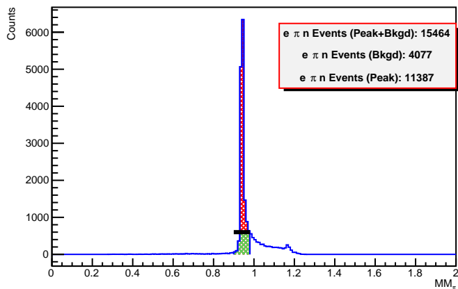
Missing Mass data (CT+accpt+aero_cut)
