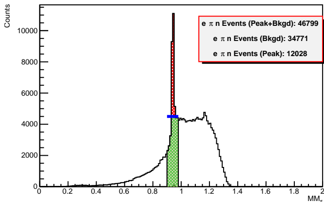
Missing Mass data (uncut)
