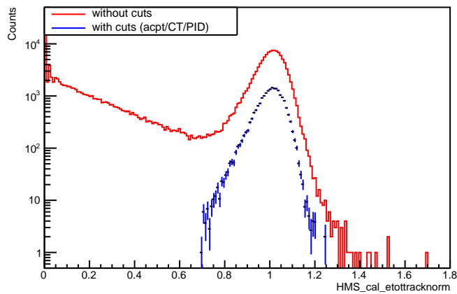
HMS cal etotracknorm (uncut)
