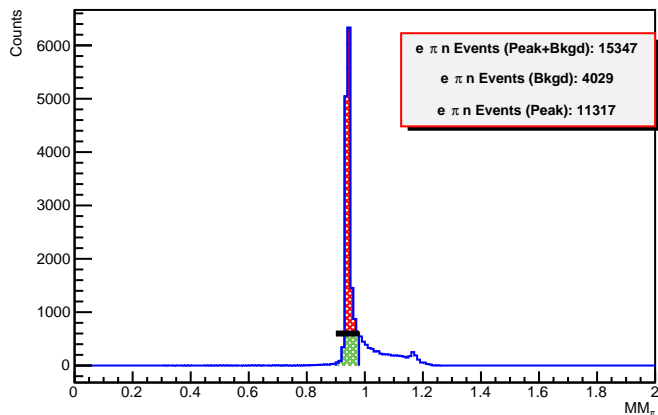
Missing Mass data (all_cut)
