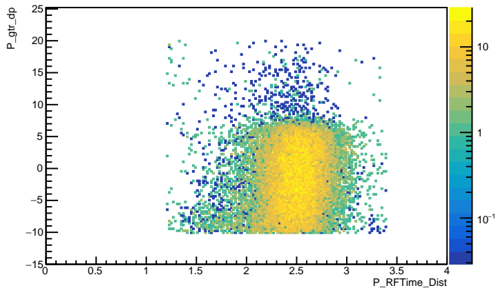
P_RTime_Dist vs P_gtr_dp (all_cut)
