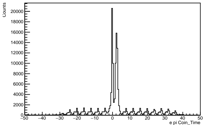
Electron-Pion CTime (uncut)
