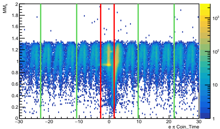
Electron-Pion CTime vs Missing Mass (uncut)
