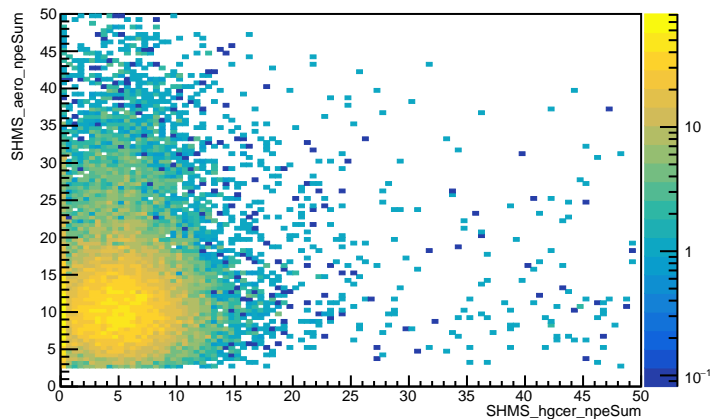
SHMS HGC npeSum vs SHMS Aero npeSum (all_cut)
