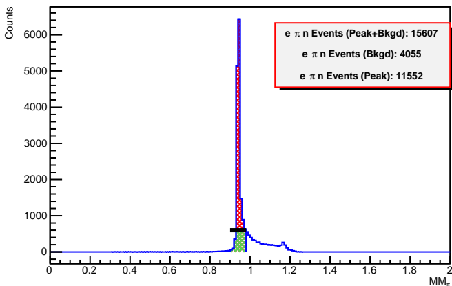
Missing Mass data (CT+accpt+RF_cut)
