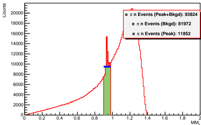
Missing Mass data (accpt_cut)
