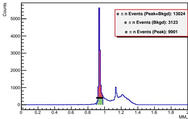
Missing Mass data (all_cut)
