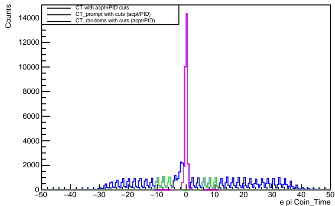
Electron-Pion CTime (accpt_PID cut)
