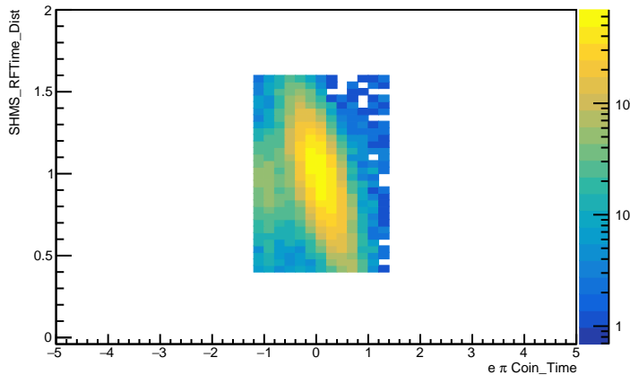
Electron-Pion CTime vs SHMS RFTIME (all_cut)
