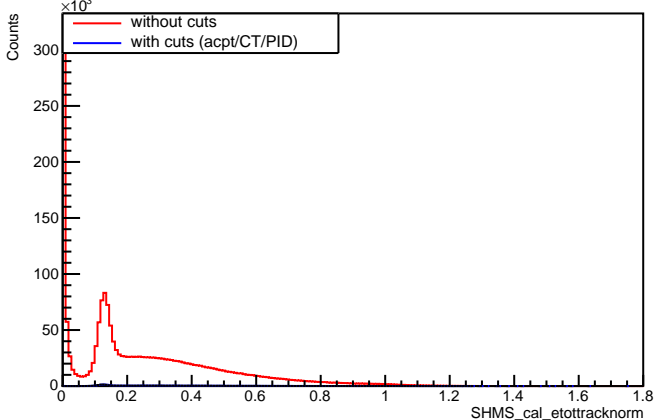
SHMS cal etotracknorm (uncut)
