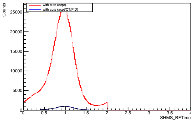
SHMS RFTIME (accpt_cut)
