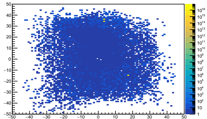
SHMS HGC NPE as fn of yAtCer vs SHMS HGC xAtCer (with cuts) profile yx projection
