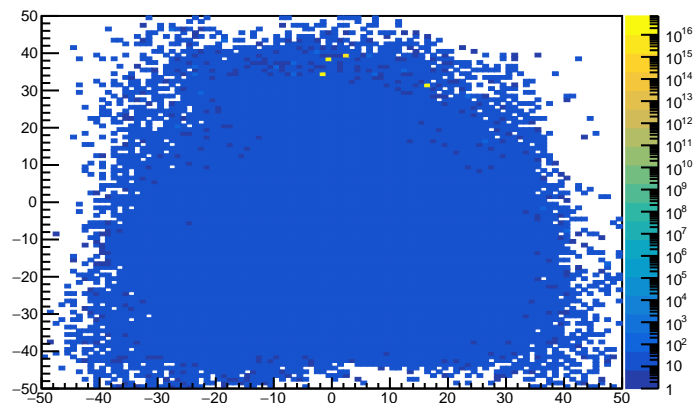
SHMS Aerogel NPE as fn of yAtCer vs xAtCer (with cuts) profile yx projection
