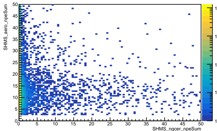
SHMS NGC npeSum vs SHMS aero npeSum (all_cut)
