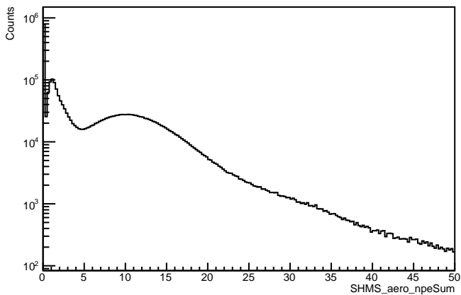
SHMS aero npeSum (uncut)
