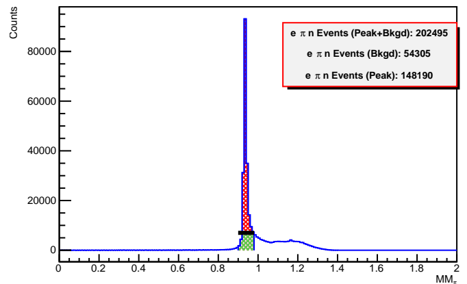
Missing Mass data (all_cut)
