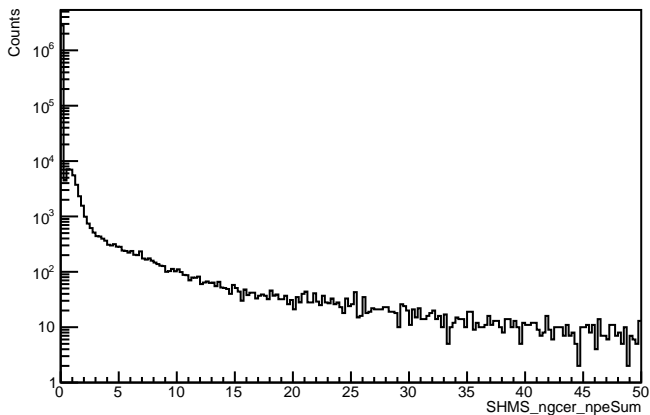
SHMS NGC npeSum (uncut)
