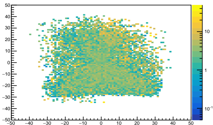
SHMS NGC NPE as fn of yAtCer vs xAtCer (no cuts) profile yx projection
