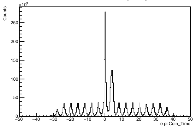
Electron-Pion CTime (uncut)
