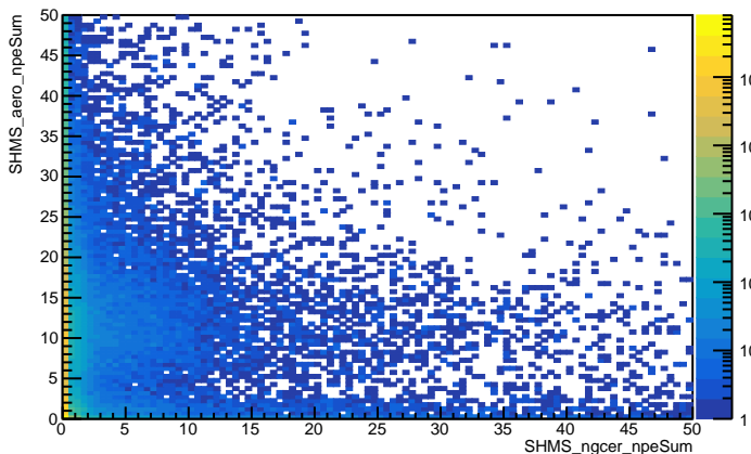
SHMS NGC npeSum vs SHMS aero npeSum (uncut)
