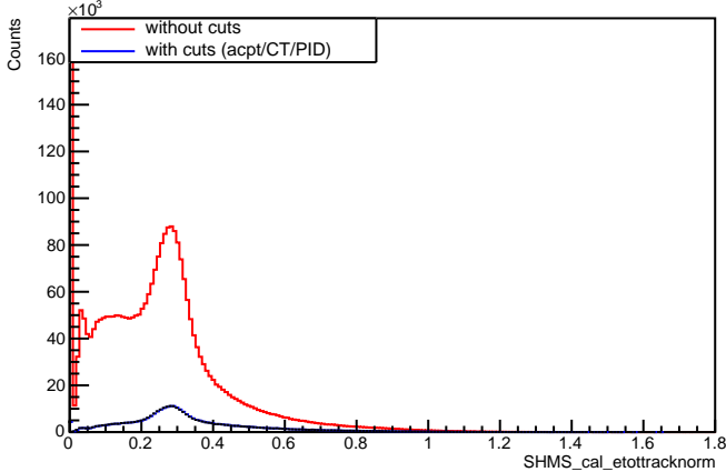
SHMS cal etottracknorm (uncut)
