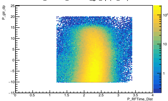
P_RTime_Dist vs P_gtr_dp (all_cut)
