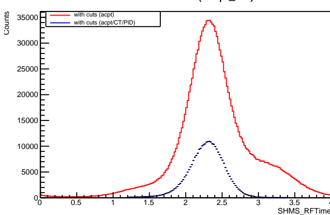
SHMS RTime (acpt_cut)
