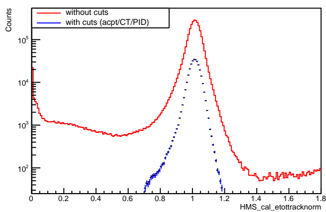
HMS cal etottracknorm (uncut)
