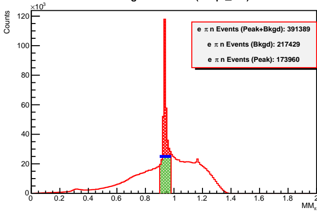
Missing Mass data (accpt_cut)
