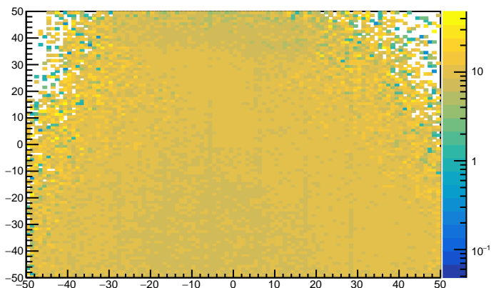
SHMS Aerogel NPE as fn of yAtCer vs xAtCer (no cuts) profile yx projection
