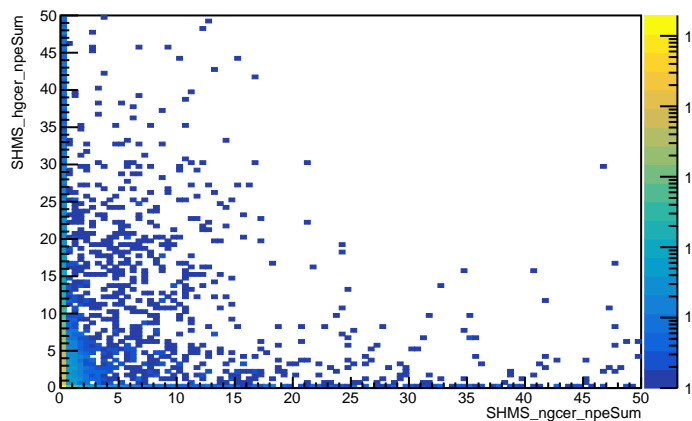
SHMS NGC npeSum vs SHMS HGC npeSum (all_cut)
