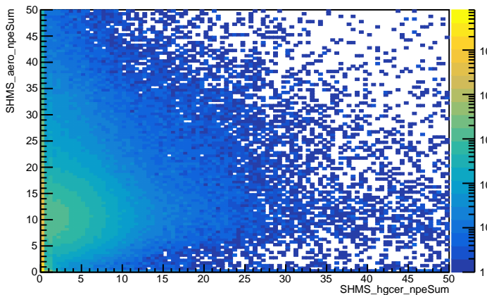
SHMS HGC npeSum vs SHMS Aero npeSum (uncut)
