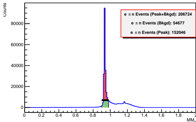
Missing Mass data (CT+accpt+RF_cut)
