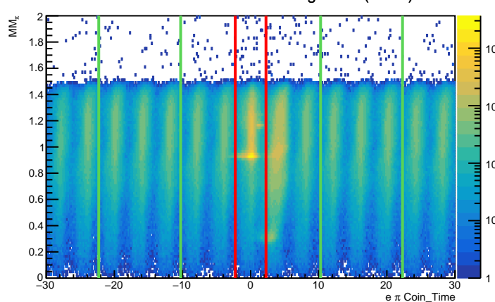
Electron-Pion CTime vs Missing Mass (uncut)
