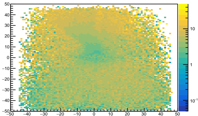
SHMS HGC NPE as fn of yAtCer vs SHMS HGC xAtCer (no cuts) profile yx projection
