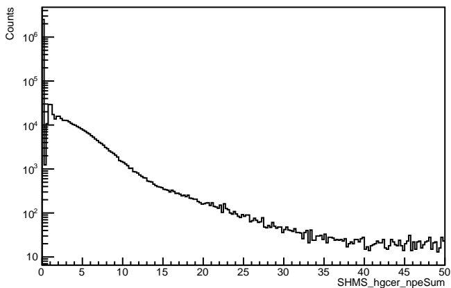
SHMS HGC npeSum (uncut)
