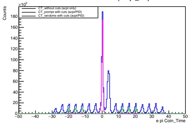
Electron-Pion CTime (acpt_cut)
