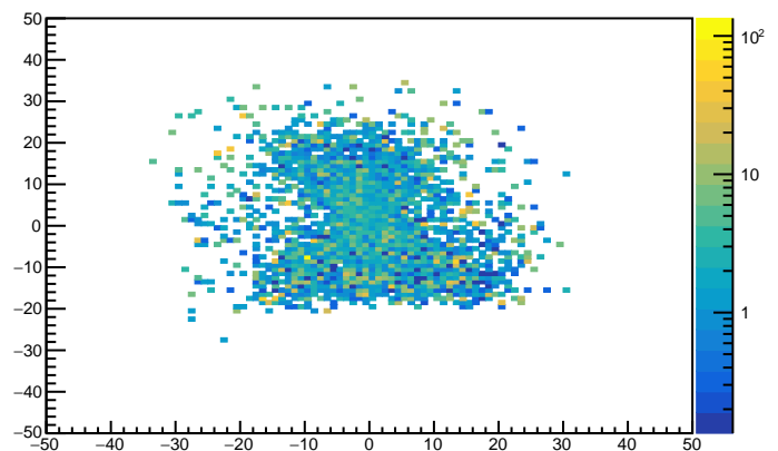
SHMS NGC NPE as fn of yAtCer vs xAtCer (with cuts) profile yx projection
