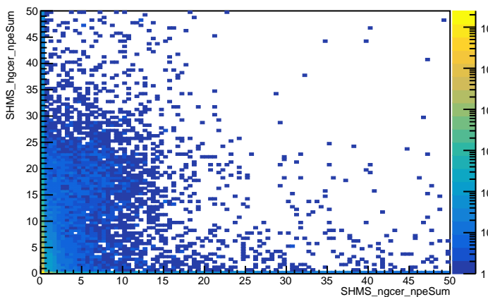
SHMS NGC npeSum vs SHMS HGC npeSum (uncut)
