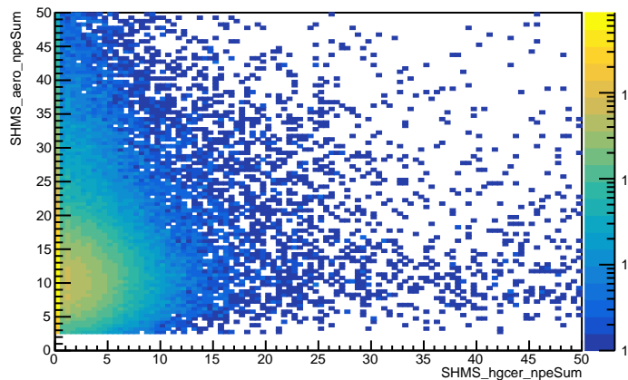
SHMS HGC npeSum vs SHMS Aero npeSum (all_cut)
