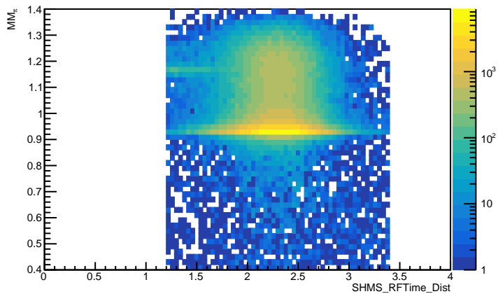
SHMS RTime vs Missing Mass (all_cut)
