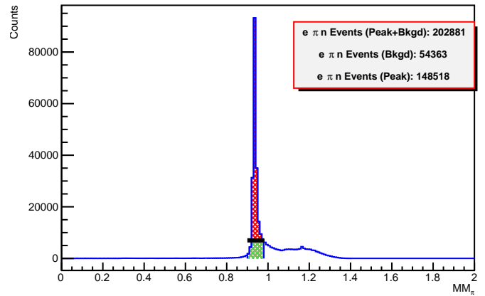
Missing Mass data (CT+accpt+aero_cut)
