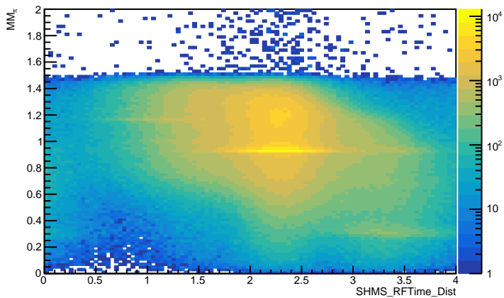
SHMS RTime vs Missing Mass (uncut)
