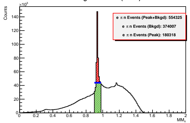
Missing Mass data (uncut)
