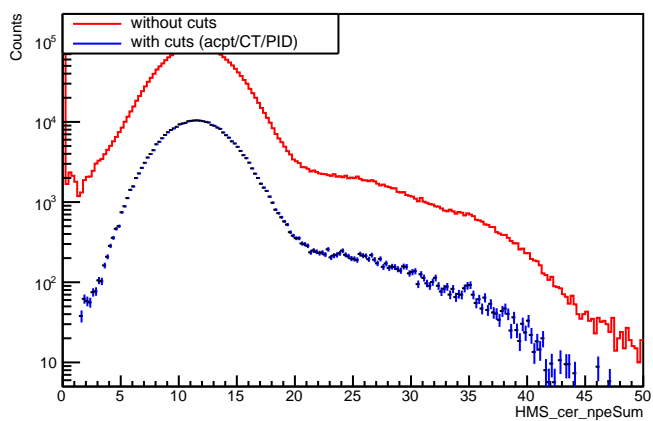
HMS cer npeSum (uncut)
