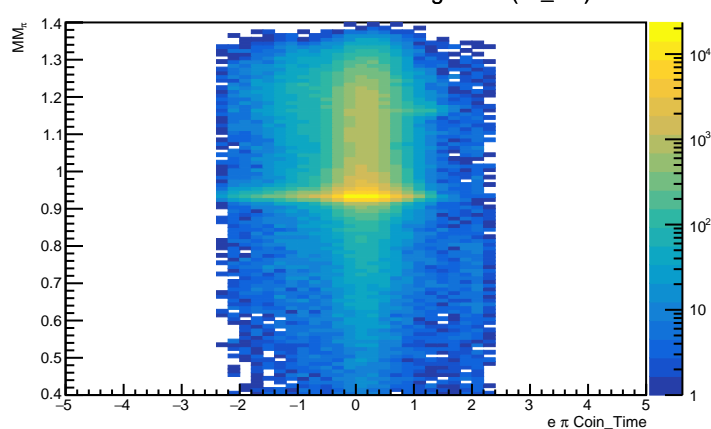
Electron-Pion CTime vs Missing Mass (all_cut)
