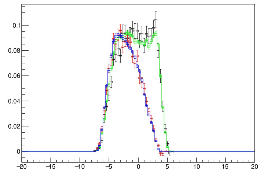
SHMS delta
