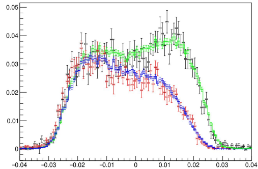
SHMS yptar
