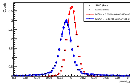
Momentum_y Distribution
