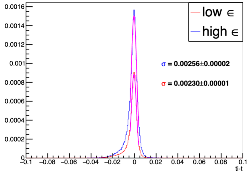
deltaT Distribution
