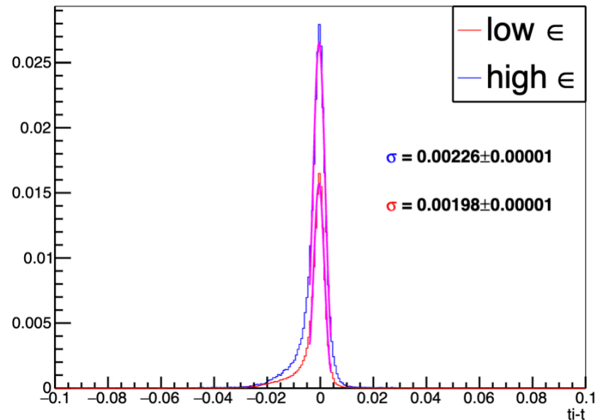
deltaT Distribution
