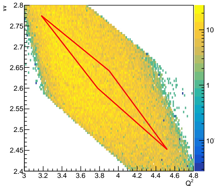
Q^2 vs W (Accpt+PID+RF+RandDummySub) Distribution
