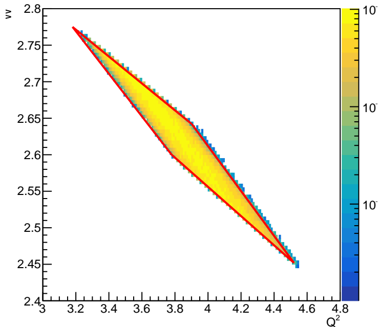
Q^2 vs W SIMC Distribution
