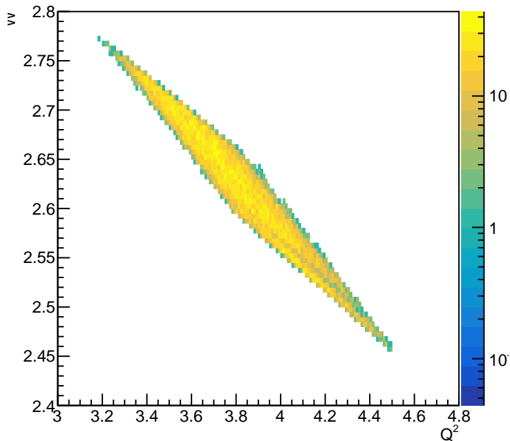
Q^2 vs W Diamond Cut Distribution
