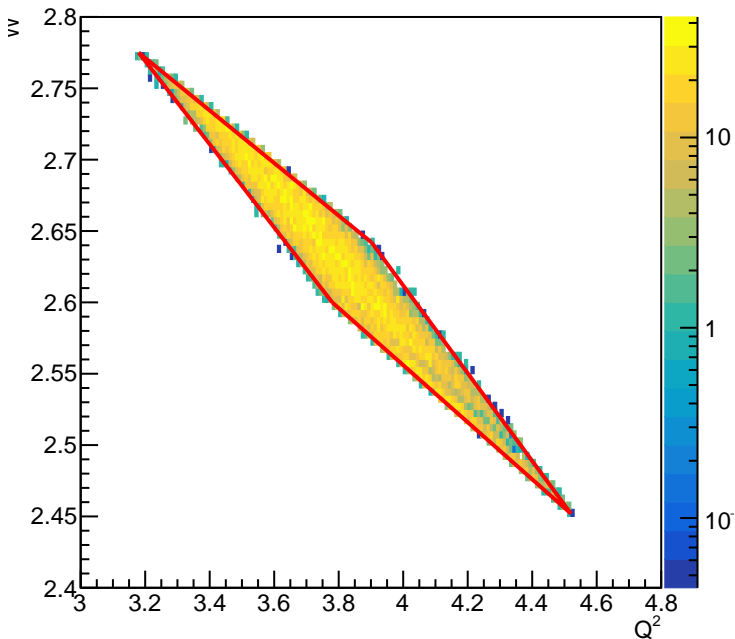
Q^2 vs W (Accpt+PID+RF+RandDummySub) Distribution
