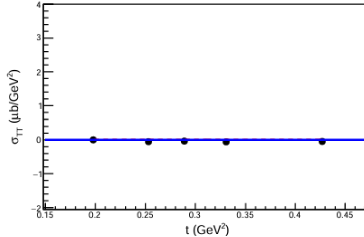
\sigma_{TT} vs t
