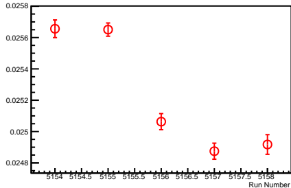
1v1 Unbiased Residual \sigma as a function of Run Number
