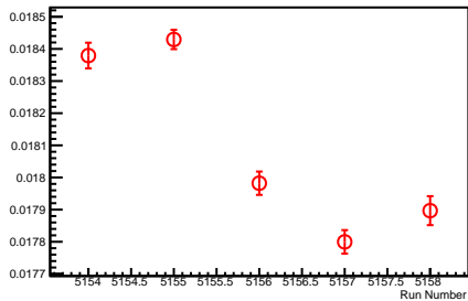
1u2 Residual \sigma as a function of Run Number
