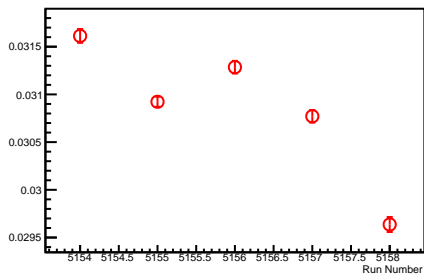
2u2 Unbiased Residual \sigma as a function of Run Number
