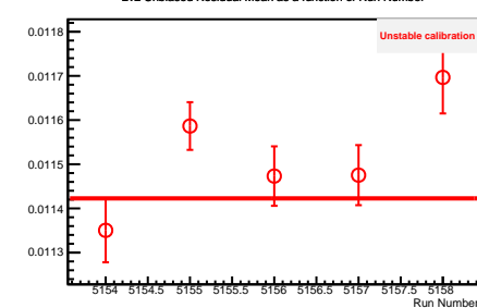
2v2 Unbiased Residual Mean as a function of Run Number
