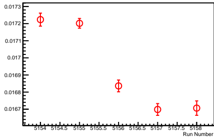
1v1 Residual \sigma as a function of Run Number
