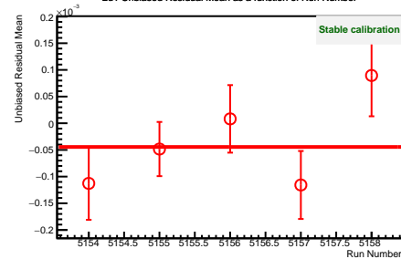
2u1 Unbiased Residual Mean as a function of Run Number
