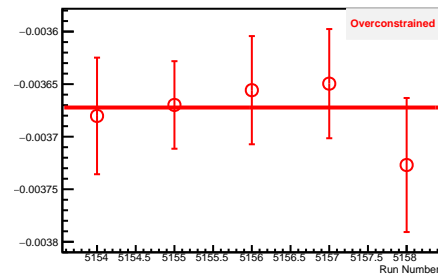
1v2 Unbiased Residual Mean as a function of Run Number
