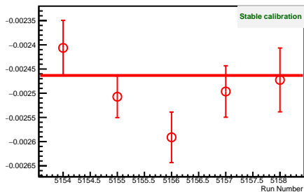
1v1 Unbiased Residual Mean as a function of Run Number
