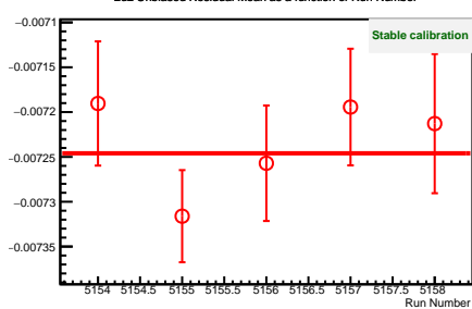
2u2 Unbiased Residual Mean as a function of Run Number
