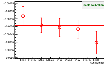
1u1 Unbiased Residual Mean as a function of Run Number
