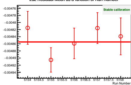
2u2 Residual Mean as a function of Run Number
