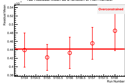
1u2 Residual Mean as a function of Run Number
