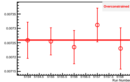
1x1 Unbiased Residual Mean as a function of Run Number
