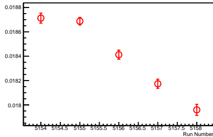
1x2 Residual \sigma as a function of Run Number
