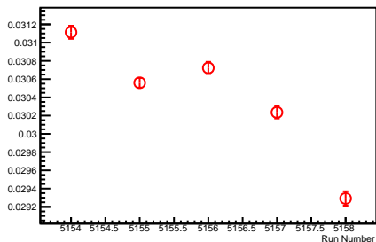
2v1 Unbiased Residual \sigma as a function of Run Number
