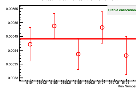
2x1 Unbiased Residual Mean as a function of Run Number
