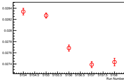
1u1 Unbiased Residual \sigma as a function of Run Number
