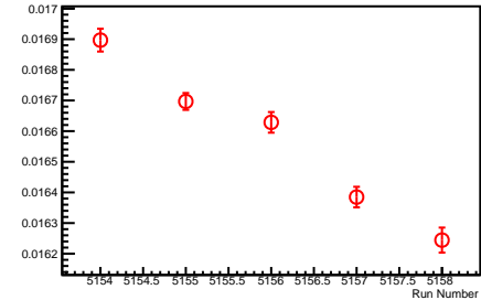
1v2 Residual \sigma as a function of Run Number
