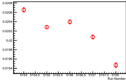
2v1 Residual \sigma as a function of Run Number
