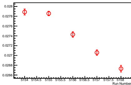
1x2 Unbiased Residual \sigma as a function of Run Number
