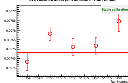
2v2 Residual Mean as a function of Run Number
