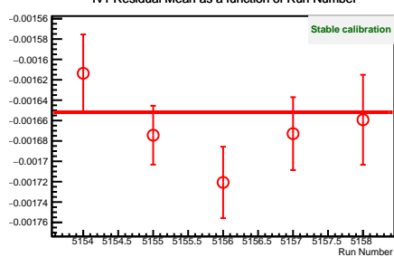
1v1 Residual Mean as a function of Run Number
