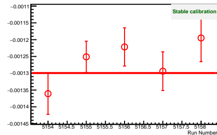
1x2 Unbiased Residual Mean as a function of Run Number
