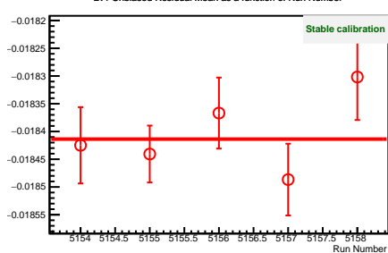
2v1 Unbiased Residual Mean as a function of Run Number
