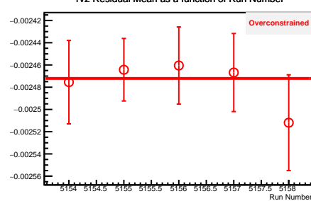
1v2 Residual Mean as a function of Run Number
