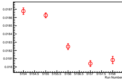
1u1 Residual \sigma as a function of Run Number
