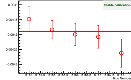
1x2 Residual Mean as a function of Run Number
