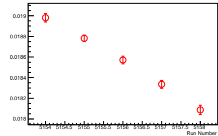
1x1 Residual \sigma as a function of Run Number
