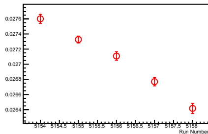
2x1 Unbiased Residual \sigma as a function of Run Number
