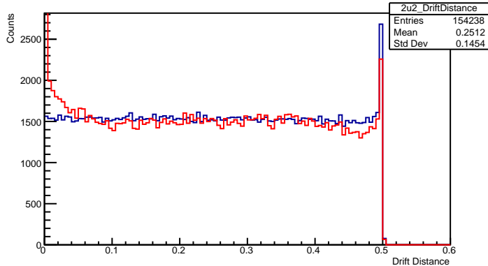
Drift Distance 2u2 Plane
