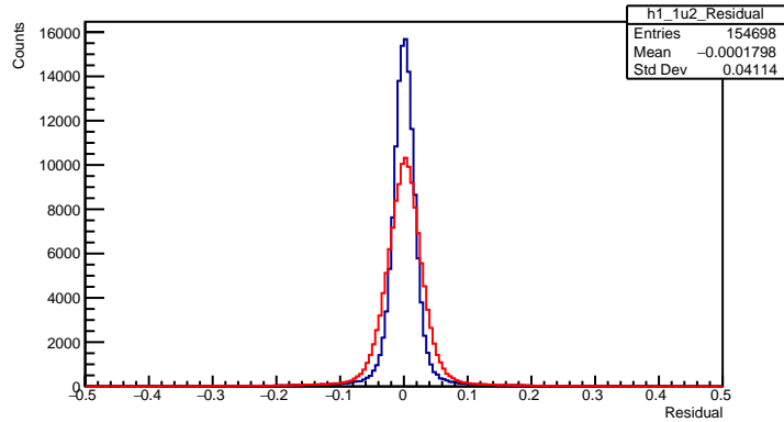
1u2 Plane Residual
