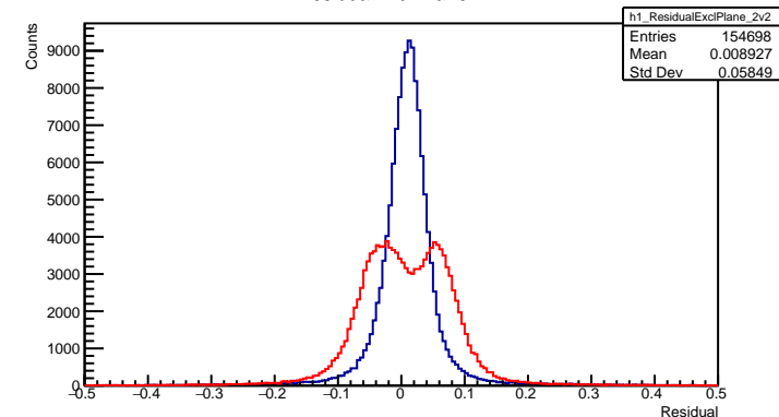
ResidualExcl Plane 2v2
