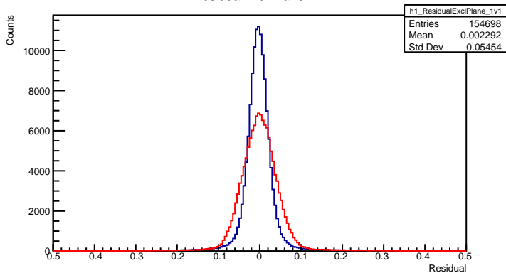
ResidualExcl Plane 1v1
