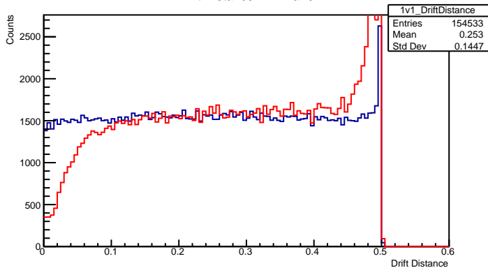
Drift Distance 1v1 Plane
