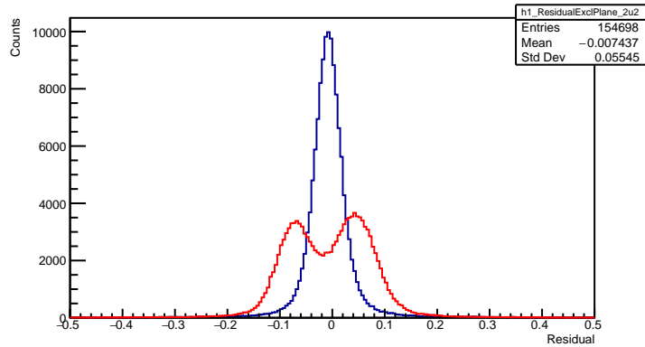
ResidualExcl Plane 2u2
