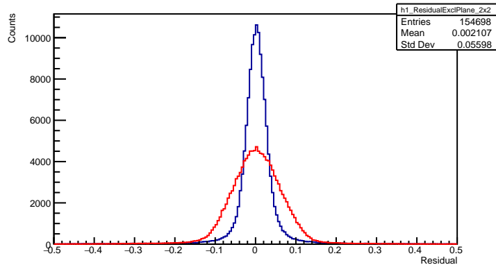
ResidualExcl Plane 2x2
