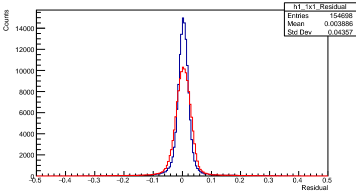
1x1 Plane Residual
