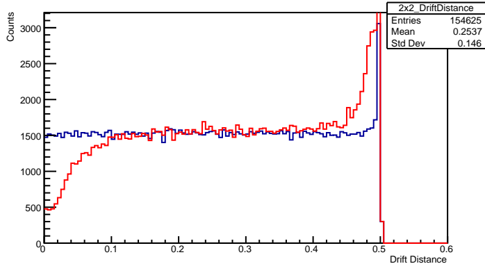
Drift Distance 2x2 Plane
