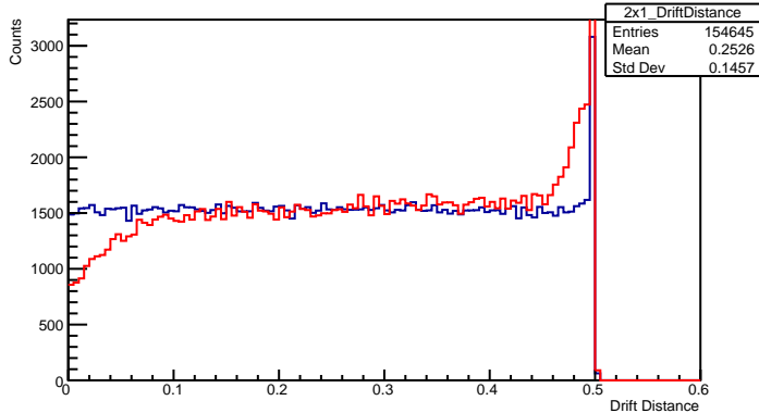
Drift Distance 2x1 Plane
