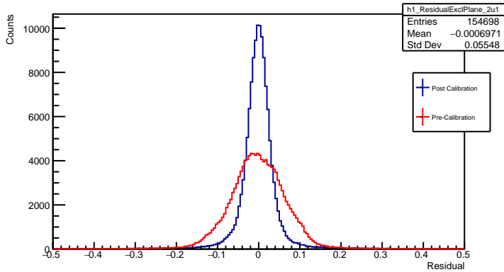
ResidualExcl Plane 2u1
