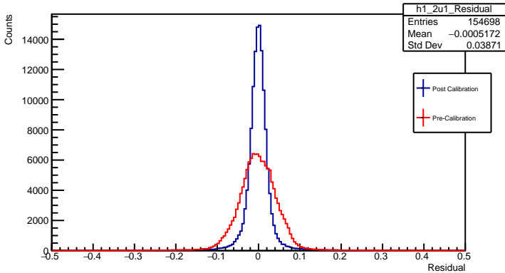
2u1 Plane Residual
