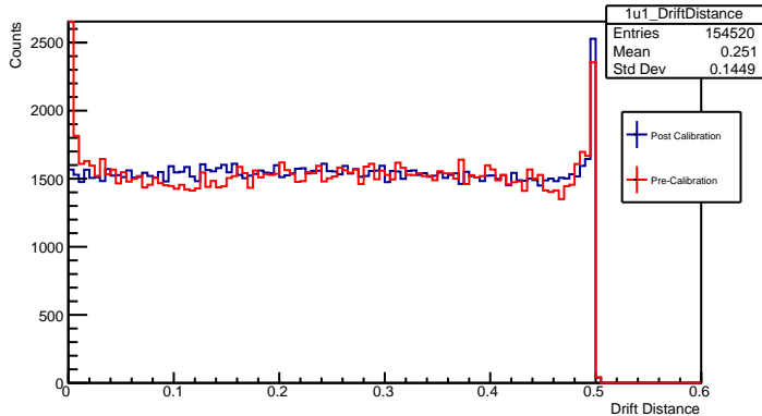
Drift Distance 1u1 Plane
