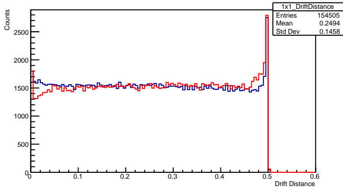
Drift Distance 1x1 Plane
