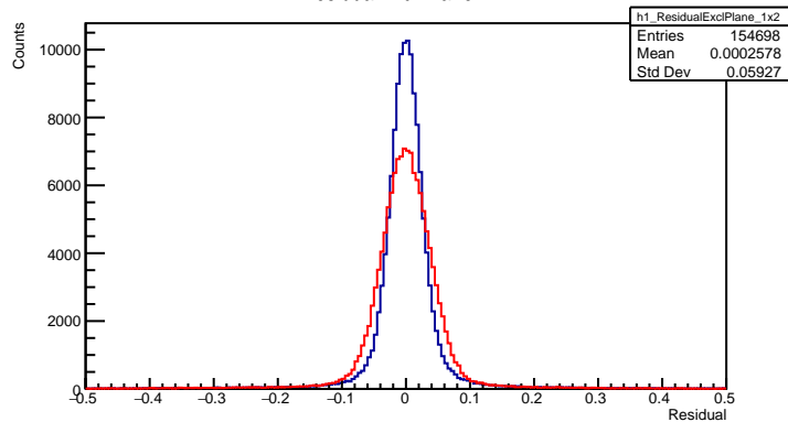
ResidualExcl Plane 1x2
