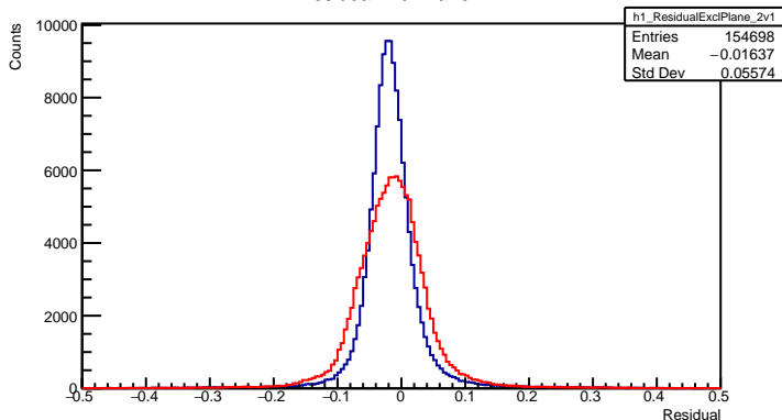
ResidualExcl Plane 2v1
