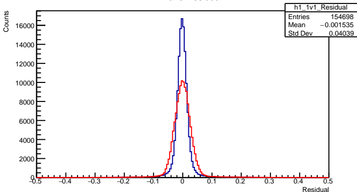
1v1 Plane Residual
