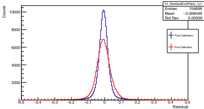
ResidualExcl Plane 1u1
