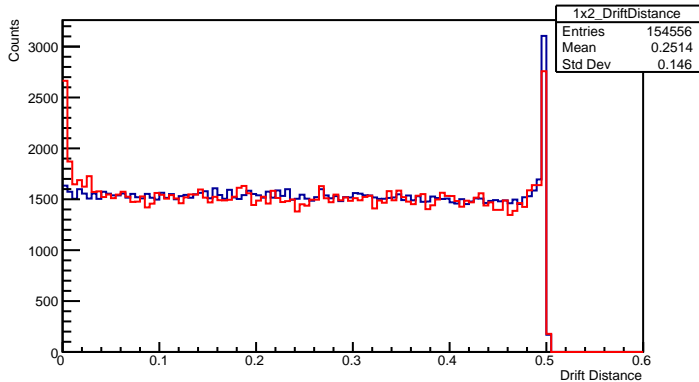
Drift Distance 1x2 Plane
