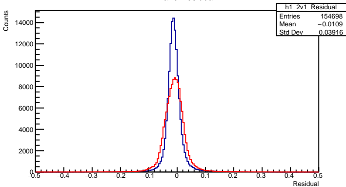
2v1 Plane Residual
