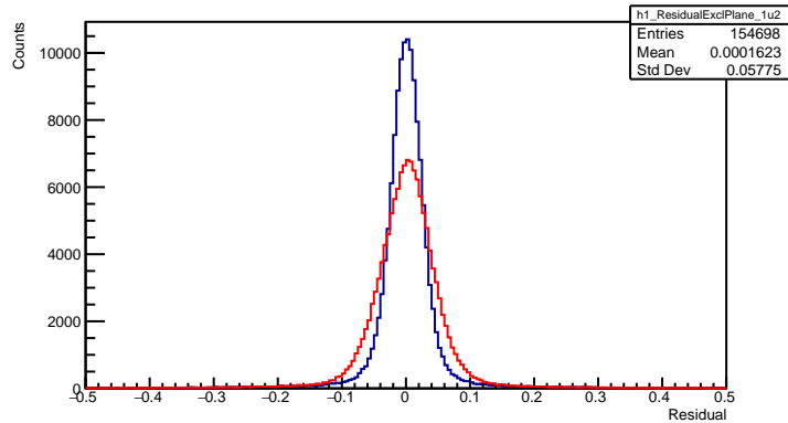
ResidualExcl Plane 1u2
