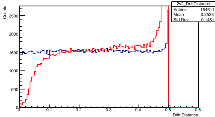
Drift Distance 2v2 Plane
