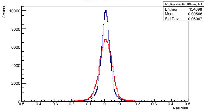
ResidualExcl Plane 1x1
