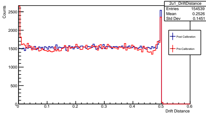
Drift Distance 2u1 Plane
