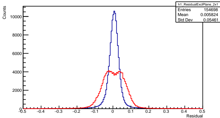
ResidualExcl Plane 2x1
