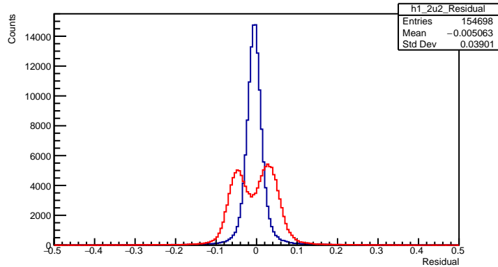
2u2 Plane Residual
