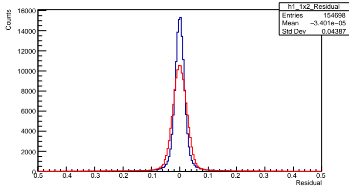
1x2 Plane Residual
