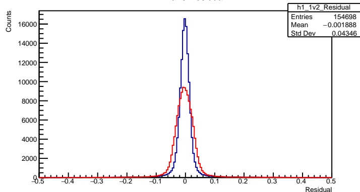
1v2 Plane Residual
