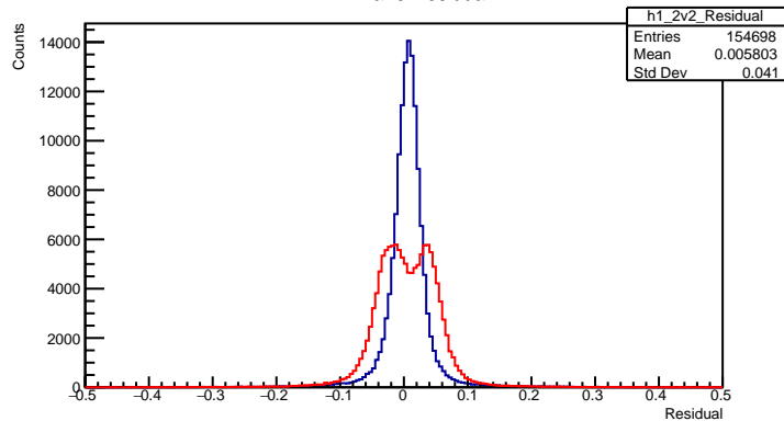
2v2 Plane Residual
