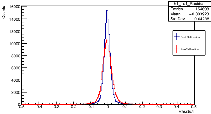
1u1 Plane Residual
