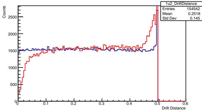
Drift Distance 1u2 Plane
