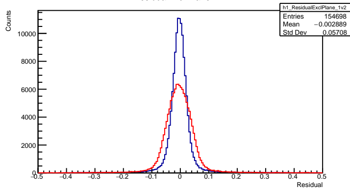
ResidualExcl Plane 1v2
