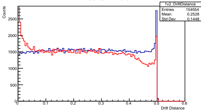
Drift Distance 1v2 Plane
