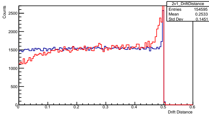
Drift Distance 2v1 Plane
