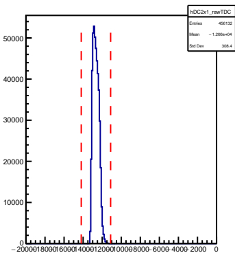
HMS DC Plane 2x1 Raw TDC
