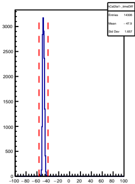
HMS Cal 2ta1- AdcTdcTimeDiff
