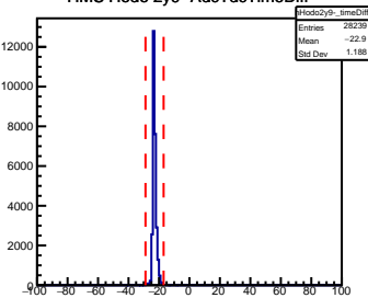
HMS Hodo 2y9- AdcTdcTimeDiff
