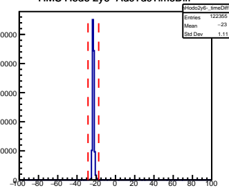
HMS Hodo 2y6- AdcTdcTimeDiff
