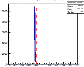
HMS Hodo 2y9+ AdcTdcTimeDiff
