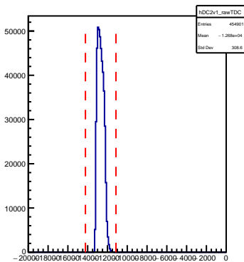
HMS DC Plane 2v1 Raw TDC
