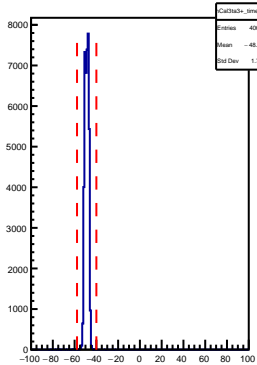
HMS Cal 3ta3+ AdcTdcTimeDiff
