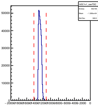
HMS DC Plane 1v1 Raw TDC
