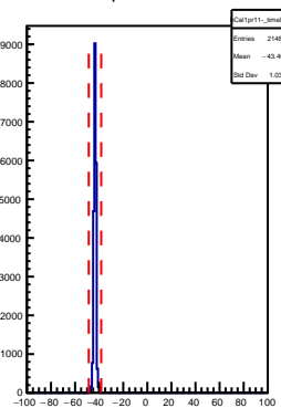
HMS Cal 1pr11- AdcTdcTimeDiff
