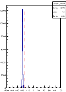
HMS Cal 1pr6+ AdcTdcTimeDiff
