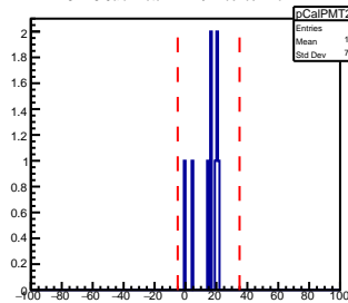
SHMS Calorimeter PMT204 AdcTdcTimeDiff
