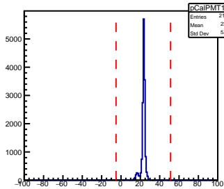
SHMS Calorimeter PMT118 AdcTdcTimeDiff
