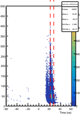
SHMS Hodo 1x8+ AdcTdcTimeDiff vs ADC Pulse Amp
