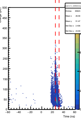
SHMS Hodo 1x11+ AdcTdcTimeDiff vs ADC Pulse Amp
