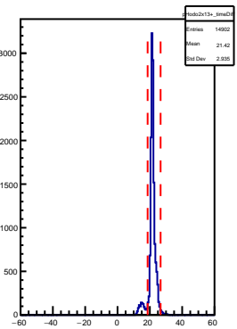
SHMS Hodo 2x13+ AdcTdcTimeDiff
