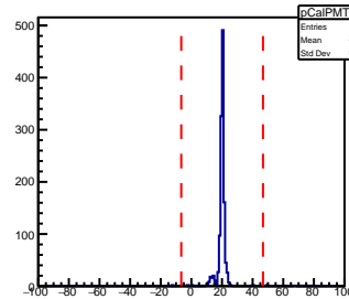
SHMS Calorimeter PMT180 AdcTdcTimeDiff
