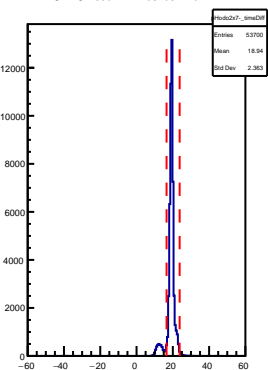
SHMS Hodo 2x7- AdcTdcTimeDiff
