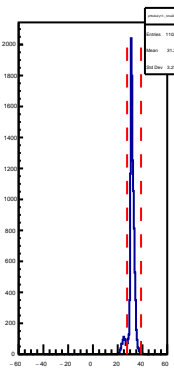
SHMS Hodo 2y17- AdcTdcTimeDiff
