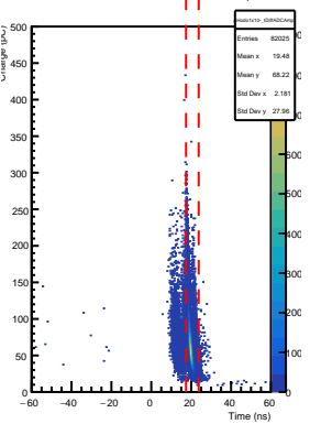
SHMS Hodo 1x10- AdcTdcTimeDiff vs ADC Pulse Amp
