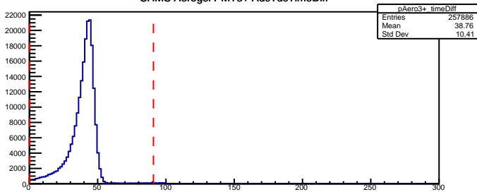
SHMS Aerogel PMT3+ AdcTdcTimeDiff
