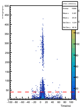
SHMS Pre-Shower PMT4- AdcTcTimeDiff vs ADC Pulse Amp
