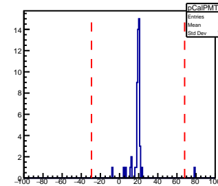
SHMS Calorimeter PMT184 AdcTdcTimeDiff
