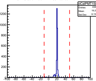
SHMS Calorimeter PMT150 AdcTdcTimeDiff
