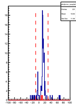
SHMS Pre-Shower PMT14+ AdcTdcTimeDiff
