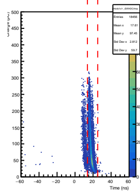
SHMS Hodo 1x1- AdcTdcTimeDiff vs ADC Pulse Amp
