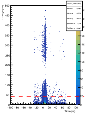
SHMS Pre-Shower PMT9- AdcTcTimeDiff vs ADC Pulse Amp
