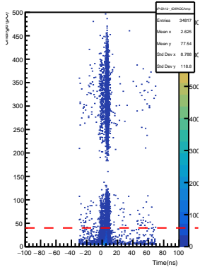
SHMS Pre-Shower PMT12- AdcTcTimeDiff vs ADC Pulse Amp
