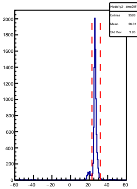
SHMS Hodo 1y2- AdcTdcTimeDiff
