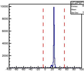
SHMS Calorimeter PMT126 AdcTdcTimeDiff
