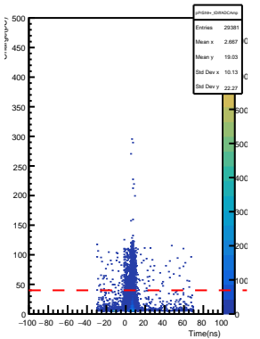
SHMS Pre-Shower PMT10+ AdcTsTimeDiff vs ADC Pulse Amp
