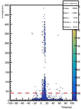
SHMS Pre-Shower PMT13- AdcTcTimeDiff vs ADC Pulse Amp
