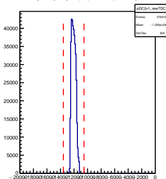
SHMS DC Plane 2v1 Raw TDC
