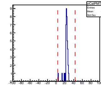
SHMS Calorimeter PMT128 AdcTdcTimeDiff
