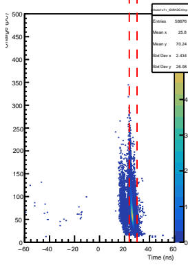
SHMS Hodo 1x7+ AdcTdcTimeDiff vs ADC Pulse Amp
