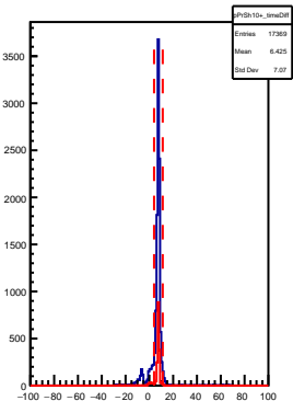
SHMS Pre-Shower PMT10+ AdcTdcTimeDiff
