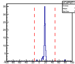
SHMS Calorimeter PMT177 AdcTdcTimeDiff
