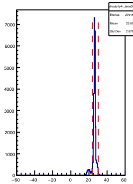
SHMS Hodo 1y4- AdcTdcTimeDiff
