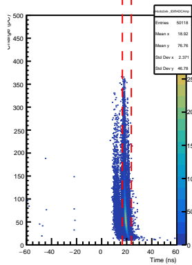
SHMS Hodo 2x6- AdcTdcTimeDiff vs ADC Pulse Amp
