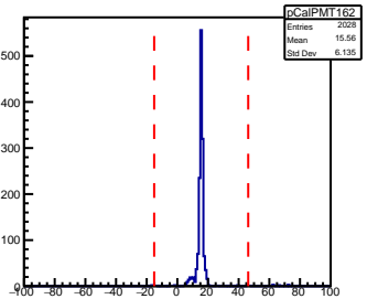
SHMS Calorimeter PMT162 AdcTdcTimeDiff
