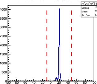
SHMS Calorimeter PMT135 AdcTdcTimeDiff
