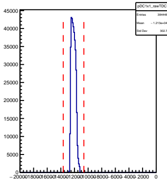
SHMS DC Plane 1x1 Raw TDC
