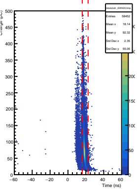
SHMS Hodo 2x8- AdcTdcTimeDiff vs ADC Pulse Amp
