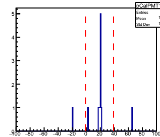
SHMS Calorimeter PMT187 AdcTdcTimeDiff
