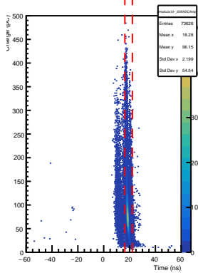
SHMS Hodo 2x10- AdcTdcTimeDiff vs ADC Pulse Amp
