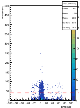
SHMS Pre-Shower PMT3- AdcTcTimeDiff vs ADC Pulse Amp
