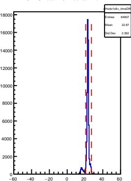
SHMS Hodo 1x8+ AdcTdcTimeDiff
