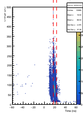
SHMS Hodo 1x6- AdcTdcTimeDiff vs ADC Pulse Amp
