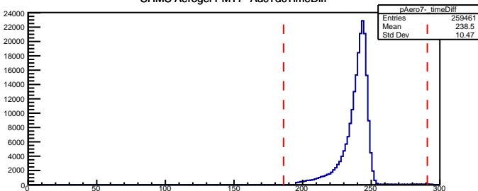
SHMS Aerogel PMT7- AdcTdcTimeDiff
