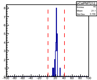
SHMS Calorimeter PMT212 AdcTdcTimeDiff
