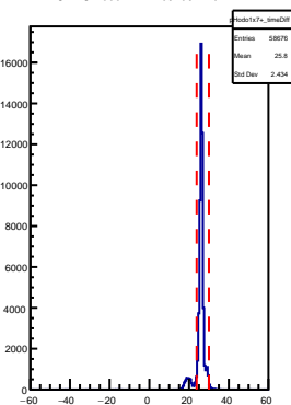
SHMS Hodo 1x7+ AdcTdcTimeDiff
