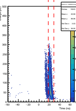
SHMS Hodo 1x1+ AdcTdcTimeDiff vs ADC Pulse Amp
