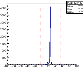
SHMS Calorimeter PMT117 AdcTdcTimeDiff
