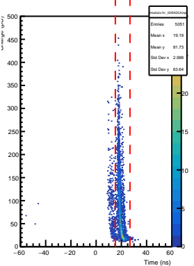
SHMS Hodo 2x14- AdcTdcTimeDiff vs ADC Pulse Amp
