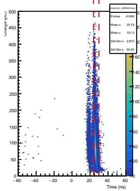
SHMS Hodo 1y5- AdcTdcTimeDiff vs ADC Pulse Amp
