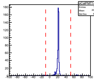
SHMS Calorimeter PMT145 AdcTdcTimeDiff
