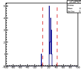
SHMS Calorimeter PMT1 AdcTdcTimeDiff
