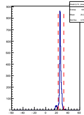
SHMS Hodo 1y13- AdcTdcTimeDiff
