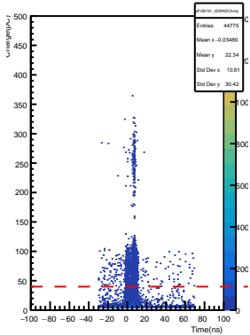
SHMS Pre-Shower PMT10- AdcTcTimeDiff vs ADC Pulse Amp
