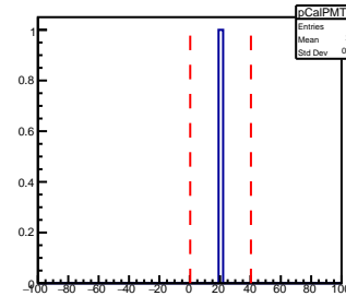
SHMS Calorimeter PMT188 AdcTdcTimeDiff
