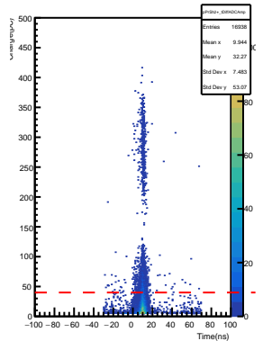
SHMS Pre-Shower PMT3+ AdcTsTimeDiff vs ADC Pulse Amp
