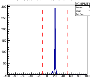
SHMS Calorimeter PMT138 AdcTdcTimeDiff
