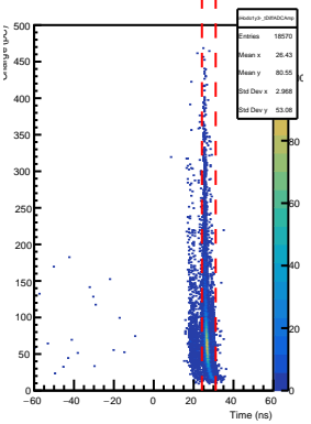
SHMS Hodo 1y3- AdcTdcTimeDiff vs ADC Pulse Amp
