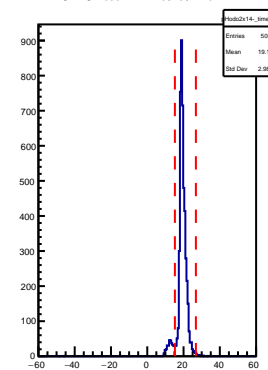
SHMS Hodo 2x14- AdcTdcTimeDiff
