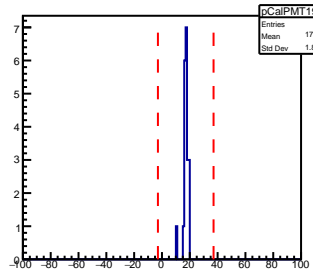
SHMS Calorimeter PMT193 AdcTdcTimeDiff
