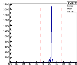
SHMS Calorimeter PMT52 AdcTdcTimeDiff
