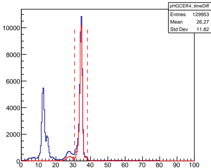
SHMS HGCer PMT4 AdcTdcTimeDiff
