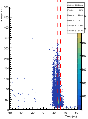
SHMS Hodo 1y8- AdcTdcTimeDiff vs ADC Pulse Amp
