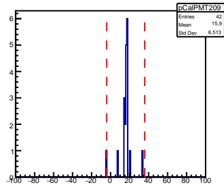
SHMS Calorimeter PMT209 AdcTdcTimeDiff
