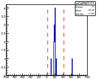
SHMS Calorimeter PMT171 AdcTdcTimeDiff
