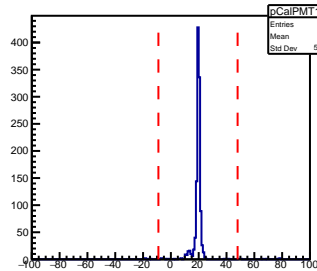
SHMS Calorimeter PMT179 AdcTdcTimeDiff
