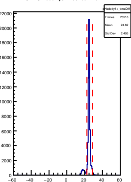
SHMS Hodo 1y6+ AdcTdcTimeDiff
