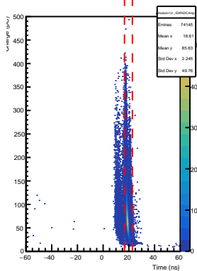
SHMS Hodo 2x12- AdcTdcTimeDiff vs ADC Pulse Amp
