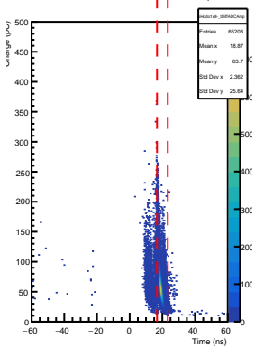
SHMS Hodo 1x8- AdcTdcTimeDiff vs ADC Pulse Amp
