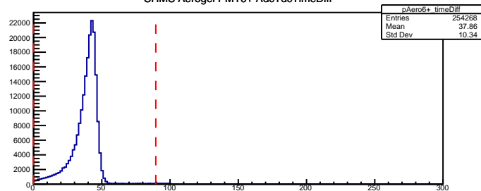
SHMS Aerogel PMT6+ AdcTdcTimeDiff
