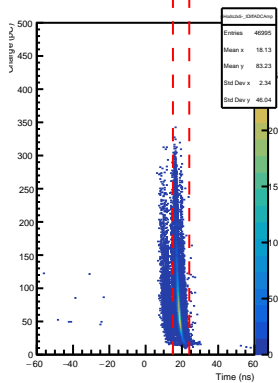
SHMS Hodo 2x5- AdcTdcTimeDiff vs ADC Pulse Amp
