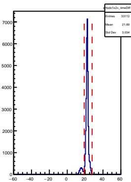
SHMS Hodo 1x2+ AdcTdcTimeDiff
