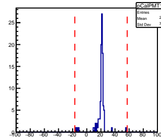
SHMS Calorimeter PMT183 AdcTdcTimeDiff
