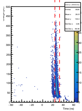
SHMS Hodo 1y2- AdcTdcTimeDiff vs ADC Pulse Amp
