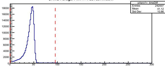
SHMS Aerogel PMT1+ AdcTdcTimeDiff
