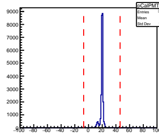
SHMS Calorimeter PMT120 AdcTdcTimeDiff
