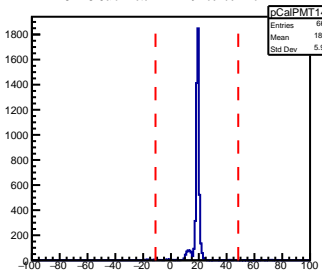
SHMS Calorimeter PMT149 AdcTdcTimeDiff
