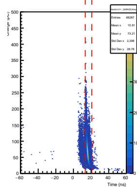
SHMS Hodo 1x11- AdcTdcTimeDiff vs ADC Pulse Amp
