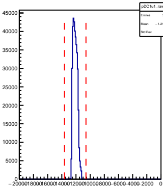
SHMS DC Plane 1u1 Raw TDC
