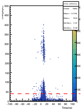
SHMS Pre-Shower PMT5- AdcTcTimeDiff vs ADC Pulse Amp
