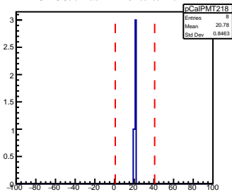
SHMS Calorimeter PMT218 AdcTdcTimeDiff
