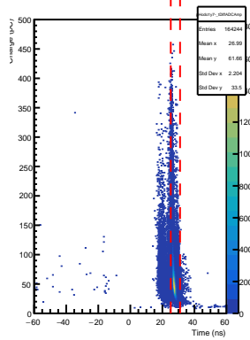
SHMS Hodo 1y7- AdcTdcTimeDiff vs ADC Pulse Amp
