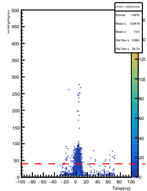
SHMS Pre-Shower PMT1+ AdcTsTimeDiff vs ADC Pulse Amp
