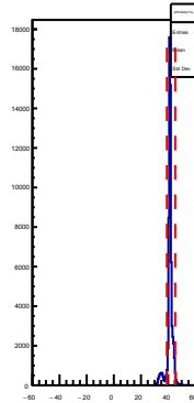
SHMS Hodo 2y13+ AdcTdcTimeDiff
