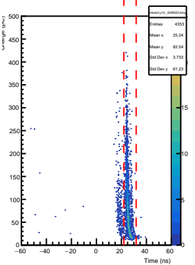
SHMS Hodo 1y13- AdcTdcTimeDiff vs ADC Pulse Amp
