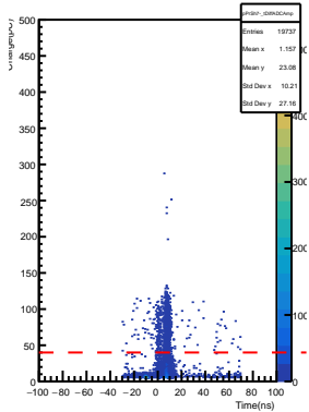
SHMS Pre-Shower PMT7- AdcTcTimeDiff vs ADC Pulse Amp
