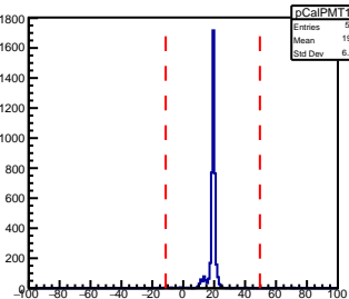
SHMS Calorimeter PMT131 AdcTdcTimeDiff
