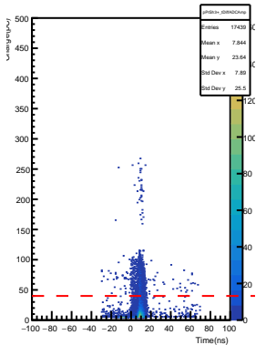
SHMS Pre-Shower PMT4+ AdcTsTimeDiff vs ADC Pulse Amp
