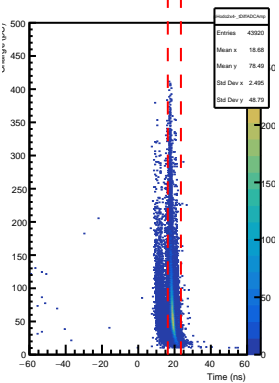
SHMS Hodo 2x4- AdcTdcTimeDiff vs ADC Pulse Amp
