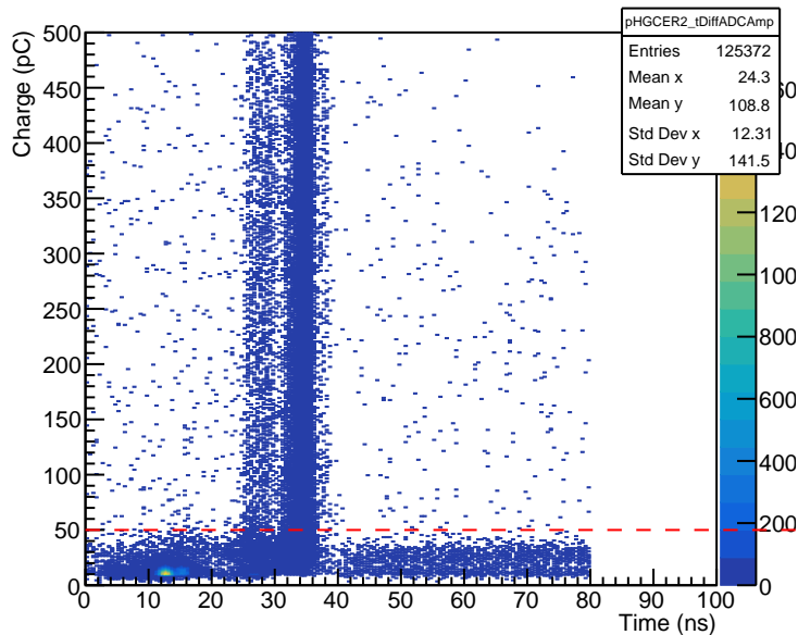
SHMS HGC ADC TDC Diff Time PMT2 vs ADC Pulse Amp
