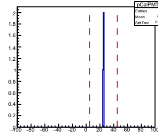
SHMS Calorimeter PMT63 AdcTdcTimeDiff
