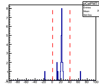
SHMS Calorimeter PMT186 AdcTdcTimeDiff
