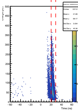
SHMS Hodo 1x2+ AdcTdcTimeDiff vs ADC Pulse Amp
