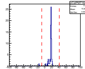
SHMS Calorimeter PMT168 AdcTdcTimeDiff
