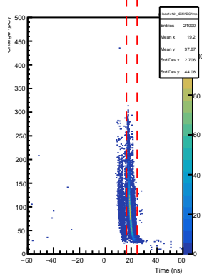
SHMS Hodo 1x12- AdcTdcTimeDiff vs ADC Pulse Amp
