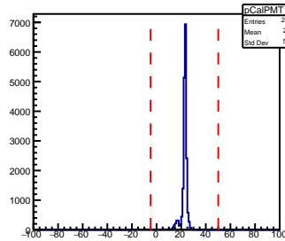
SHMS Calorimeter PMT119 AdcTdcTimeDiff
