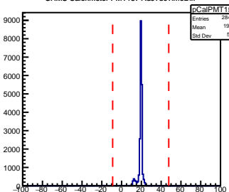
SHMS Calorimeter PMT157 AdcTdcTimeDiff
