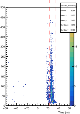
SHMS Hodo 1x13+ AdcTdcTimeDiff vs ADC Pulse Amp
