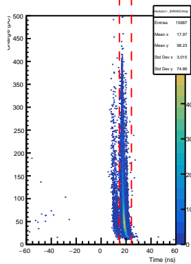
SHMS Hodo 2x1- AdcTdcTimeDiff vs ADC Pulse Amp
