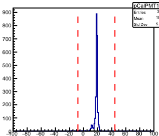
SHMS Calorimeter PMT130 AdcTdcTimeDiff
