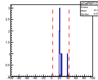
SHMS Calorimeter PMT172 AdcTdcTimeDiff
