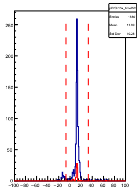
SHMS Pre-Shower PMT13+ AdcTdcTimeDiff
