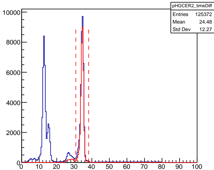
SHMS HGCer PMT2 AdcTdcTimeDiff
