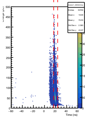
SHMS Hodo 2x7- AdcTdcTimeDiff vs ADC Pulse Amp
