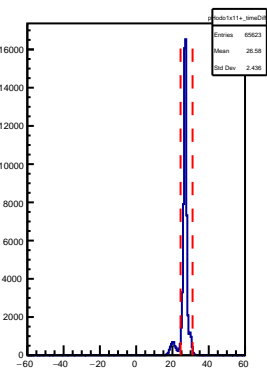
SHMS Hodo 1x11+ AdcTdcTimeDiff
