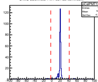
SHMS Calorimeter PMT153 AdcTdcTimeDiff
