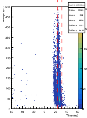
SHMS Hodo 1y10- AdcTdcTimeDiff vs ADC Pulse Amp
