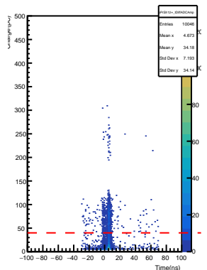
SHMS Pre-Shower PMT13+ AdcTsTimeDiff vs ADC Pulse Amp
