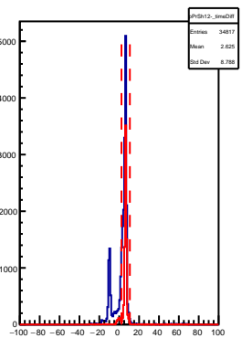
SHMS Pre-Shower PMT12- AdcTdcTimeDiff
