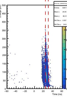
SHMS Hodo 1x6+ AdcTdcTimeDiff vs ADC Pulse Amp
