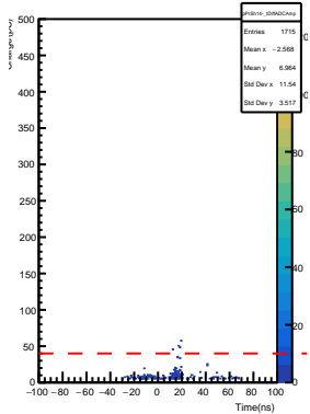
SHMS Pre-Shower PMT14- AdcTcTimeDiff vs ADC Pulse Amp
