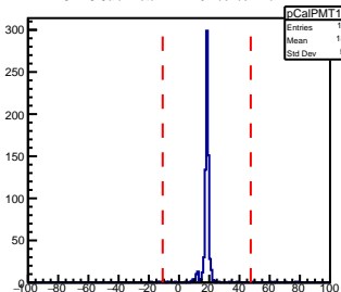
SHMS Calorimeter PMT143 AdcTdcTimeDiff
