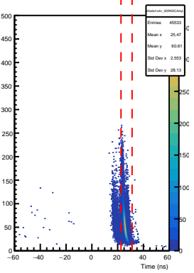
SHMS Hodo 1x4+ AdcTdcTimeDiff vs ADC Pulse Amp
