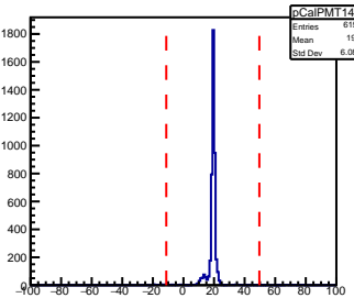
SHMS Calorimeter PMT147 AdcTdcTimeDiff
