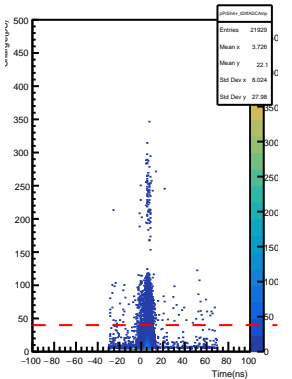
SHMS Pre-Shower PMT5+ AdcTsTimeDiff vs ADC Pulse Amp
