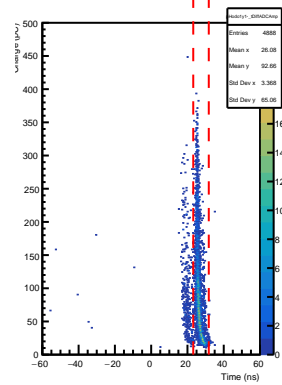
SHMS Hodo 1y1- AdcTdcTimeDiff vs ADC Pulse Amp
