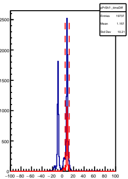
SHMS Pre-Shower PMT7- AdcTdcTimeDiff
