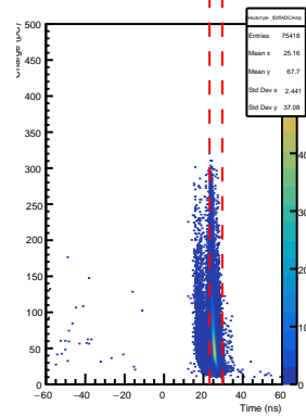
SHMS Hodo 1y6- AdcTdcTimeDiff vs ADC Pulse Amp
