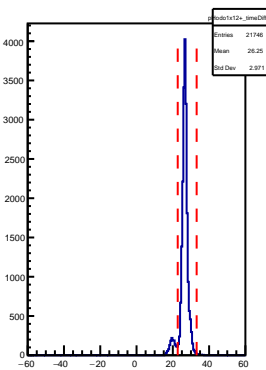
SHMS Hodo 1x12+ AdcTdcTimeDiff
