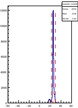
SHMS Hodo 2x6+ AdcTdcTimeDiff
