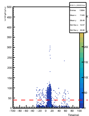
SHMS Pre-Shower PMT12+ AdcTsTimeDiff vs ADC Pulse Amp
