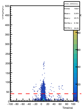
SHMS Pre-Shower PMT2- AdcTcTimeDiff vs ADC Pulse Amp
