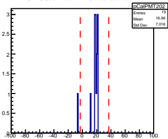
SHMS Calorimeter PMT202 AdcTdcTimeDiff
