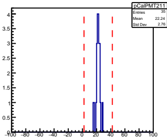
SHMS Calorimeter PMT211 AdcTdcTimeDiff
