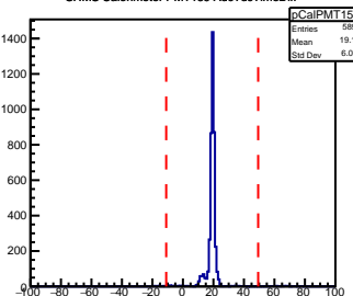
SHMS Calorimeter PMT159 AdcTdcTimeDiff
