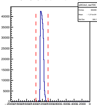
SHMS DC Plane 2x2 Raw TDC
