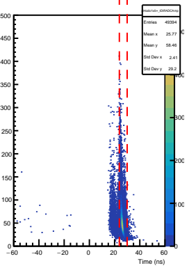
SHMS Hodo 1x5+ AdcTdcTimeDiff vs ADC Pulse Amp
