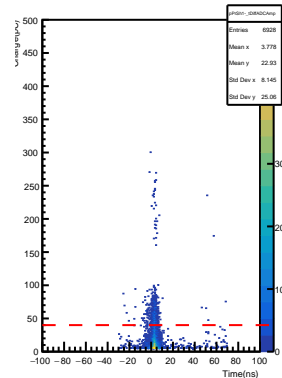
SHMS Pre-Shower PMT1- AdcTcTimeDiff vs ADC Pulse Amp
