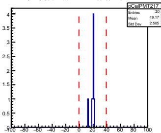
SHMS Calorimeter PMT217 AdcTdcTimeDiff
