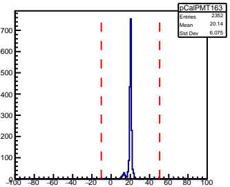
SHMS Calorimeter PMT163 AdcTdcTimeDiff
