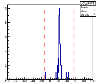
SHMS Calorimeter PMT199 AdcTdcTimeDiff
